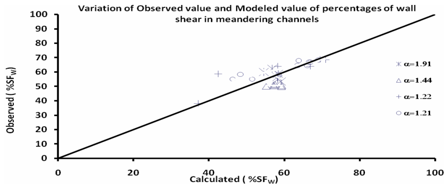
Fig. 7. Variation of Observed and Modeled Value of Wall Shear in Meandering Channel
