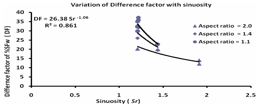
Fig. 6. Variation of Difference Factor of Wall Shear with Sinuosity
