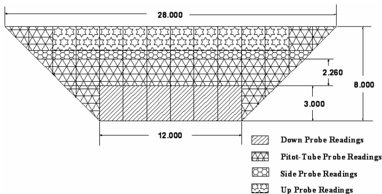
Fig. 1. Detailed Skeleton of the Probes Limit
