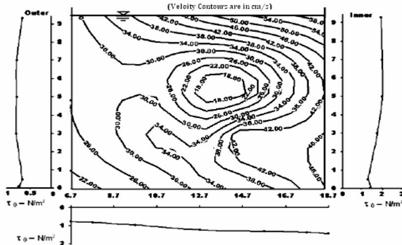
Fig. 3. Flow depth ( h' ) = 9.34 cm (Type-I Meandering Channel)
