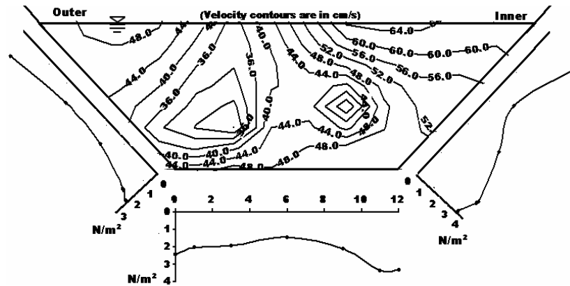
Fig. 4. Flow depth ( h' ) = 7.33 cm (Type-II Meandering Channel)
