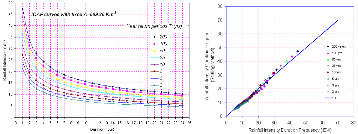
Figure 4 The IDAF curves constructed by the scaling method and comparison with traditional method for the A=569 \text{ km}^2
