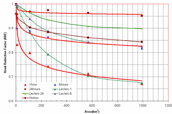
Figure 5 The areal reduction factor derived based on the scale invariance of rainfall
