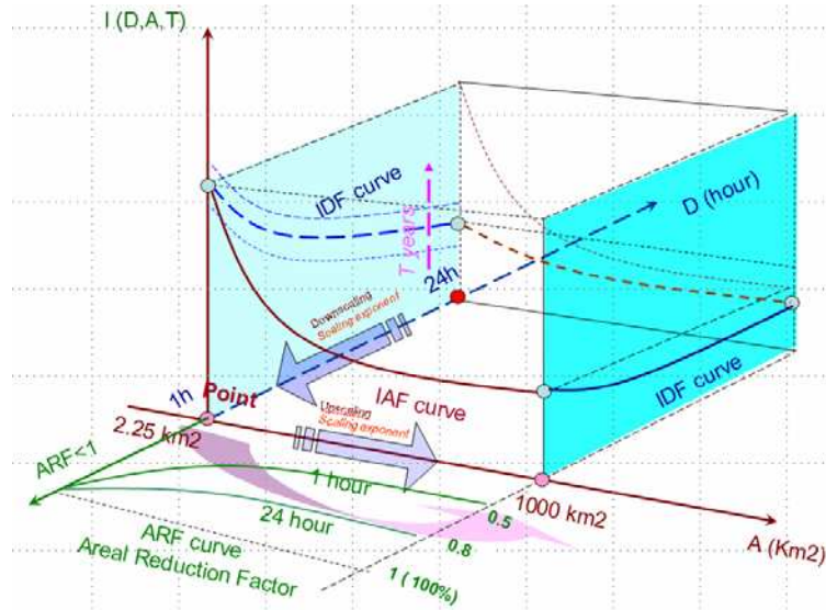
Figure 1 Derivation of intensity-duration-frequency curves and areal reduction factor.
