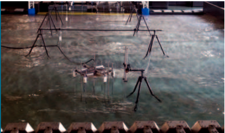
Figure 5. Directionally spread and oblique wave experiment in the wave basin at Flanders Hydraulics Research
