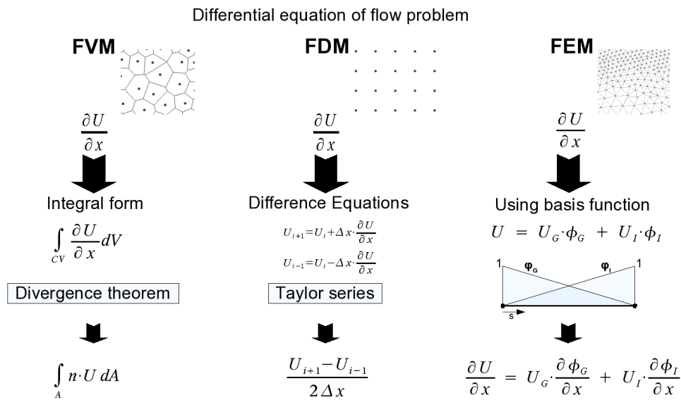
Figure 1: The most commonly used numerical methods and their essential differences
