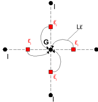
Figure 6: The Local Residual Correction of a finite difference node
