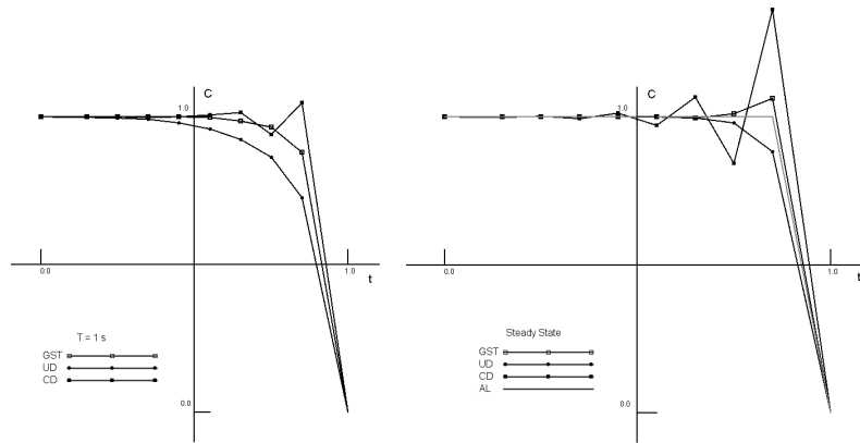
Figure 8: Analytical (AL) and numerical solutions of the advection dominant problem
