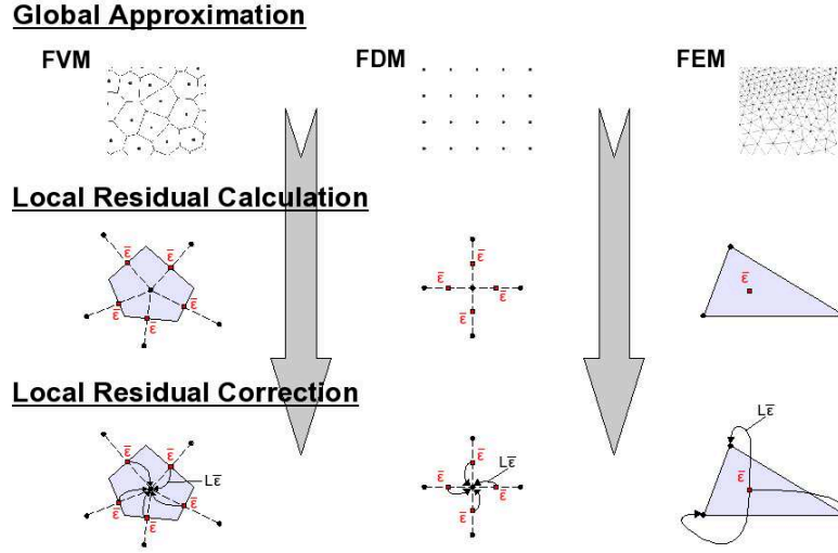
Figure 3: Sketch of the GST steps for the FVM, FDM and FEM
