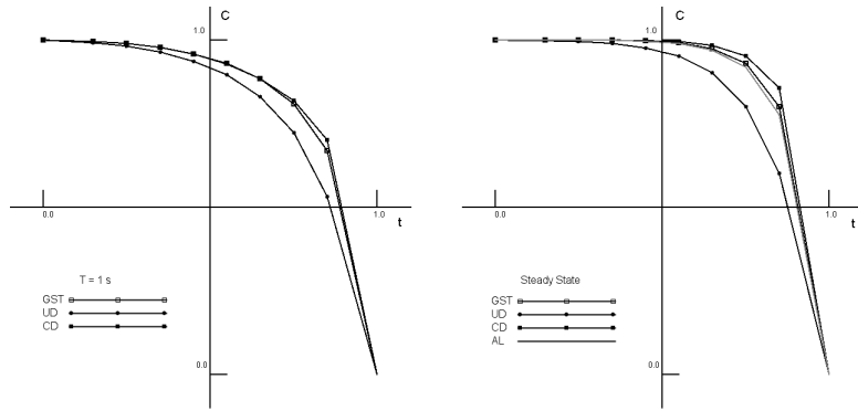
Figure 7: Analytical (AL) and numerical solutions of the diffusion dominant problem
