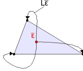
Figure 4: The Local Residual Correction of a finite element
