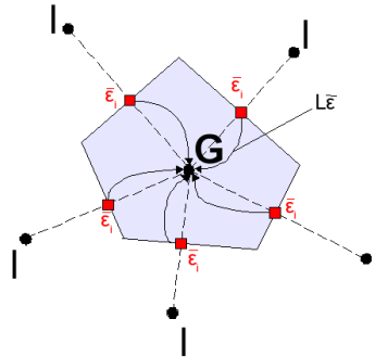
Figure 5: The Local Residual Correction of a finite volume
