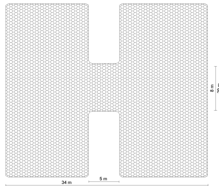
Figure 9: The computational domain with 4231 voronoi-region finite volumes
