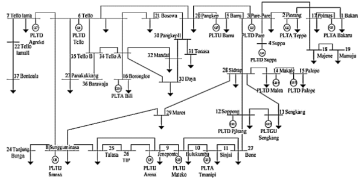
Gambar 4. 5 Single Line Diagram Sistem Kelistrikan Sulselbar
