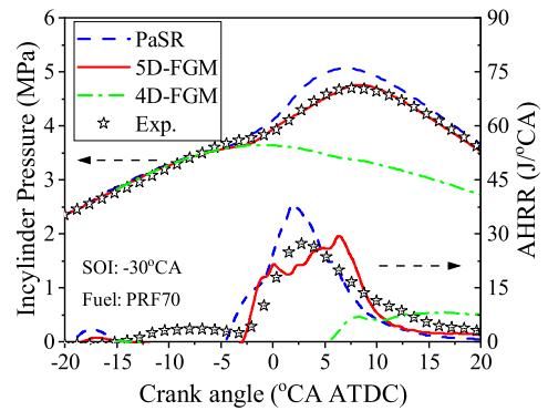
Fig. 2. In-cylinder pressure and apparent heat release rate (AHRR) from the simulations and experiments.
