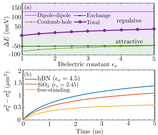
FIG. 5. Impact of dielectric environment on spectral shift and transport of interlayer excitons at a fixed exciton density n_x = 5 \times 10^{12} cm -2 . (a) Screening dependence of the energy renormalization \Delta E distinguishing different contributions. The total exciton-exciton interaction (purple line) shows only a weak dependence that can be traced back to the Coulomb-hole contribution (bright green line). (b) Temporal evolution of the variance \sigma_t^2 - \sigma_0^2 as a function of time for different surrounding substrates.
