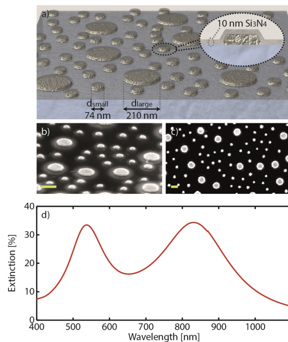
Figure 2. Dual-band nanoplasmonic ruler design and optical spectra. (a) Artist's rendition of the sensor surface comprising a quasi-random array of two distinct populations of Ag nanodisks with diameters d_{\text{small}} = 74 nm and d_{\text{large}} = 210 nm, both with a height h = 20 nm, covered with a conformal 10 nm thin \text{Si}_3\text{N}_4 coating (inset). (b) Tilted and (c) normal incidence SEM images of the corresponding nanostructured surface. Note that the imaged sensor is not coated with \text{Si}_3\text{N}_4 for better image contrast. Scale bars are 200 nm. (d) Optical extinction spectra of the dual-band nanoplasmonic ruler sensor characterized by two spectrally distinctly separated peaks with identical intensities.
