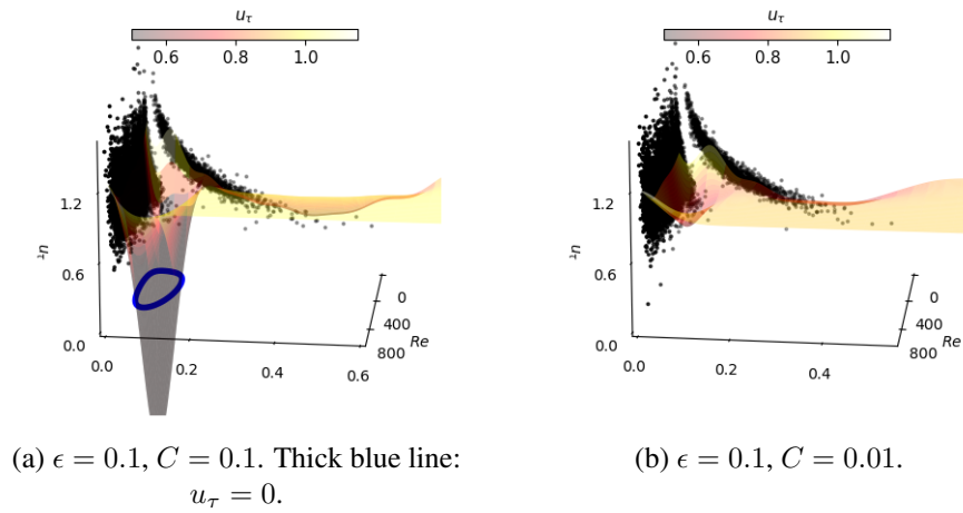
Figure 6: Predicted friction velocity with svr using low y^+ data, see Table 1. 3D view. \bullet : Predicted friction velocity; 3D surface: hyperplane colored with u_\tau
