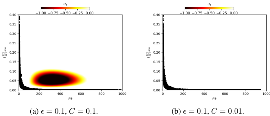
Figure 7: Predicted friction velocity with svr using low y^+ data, see Table 2. 2D view. \bullet : Predicted friction velocity; colored surface: u_\tau < 0 .
