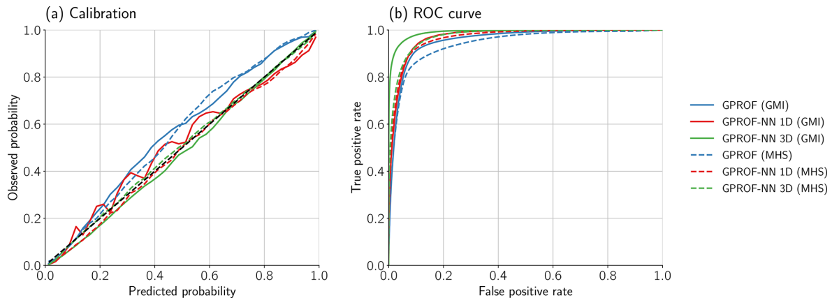
Figure 9. Calibration (a) and receiver operating characteristic (ROC, b) for the predicted probability of precipitation.
