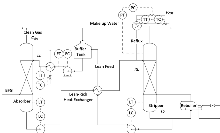
Fig. 2. Process diagram of the capture unit used to treat the blast furnace gas (BFG). The five main process variables analyzed in this work are shown in italics . The regulatory control loops are shown as dashed lines. The first letter indicates the controlled variable as follows: L, level; T, temperature; F, flow; and P, pressure. The second letter indicates the type of unit: T, transmission; C, controller.
