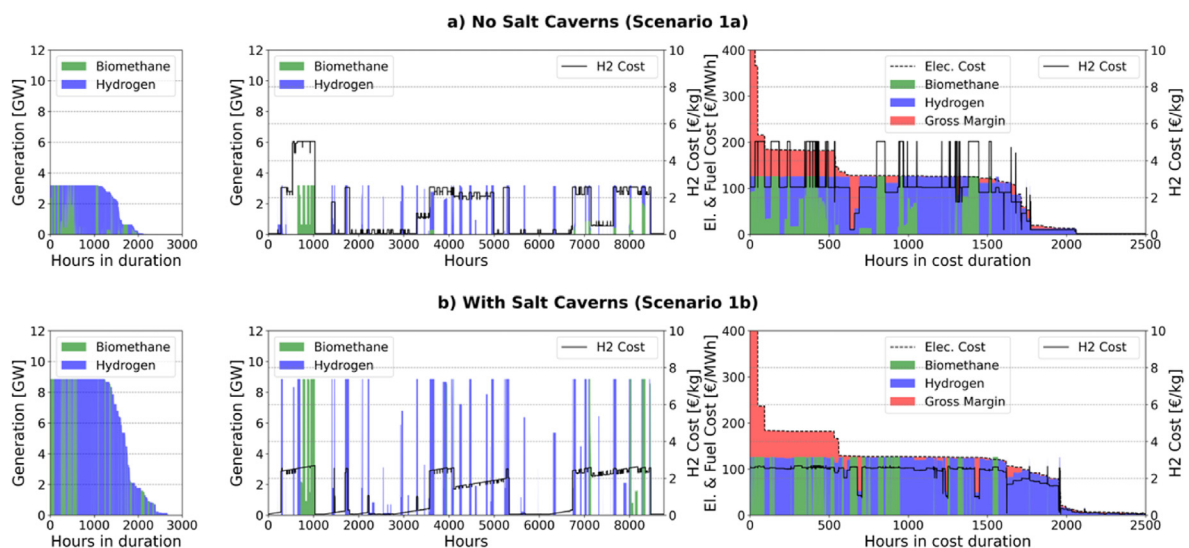
Fig. 2 – Operation of CCGTs with 100% hydrogen capability in UK1 for Scenarios 1a and 1b, where salt caverns are excluded in the modeling in a) and included in b). The biomass cost is 40 €/MWh and the availability is 20%.
