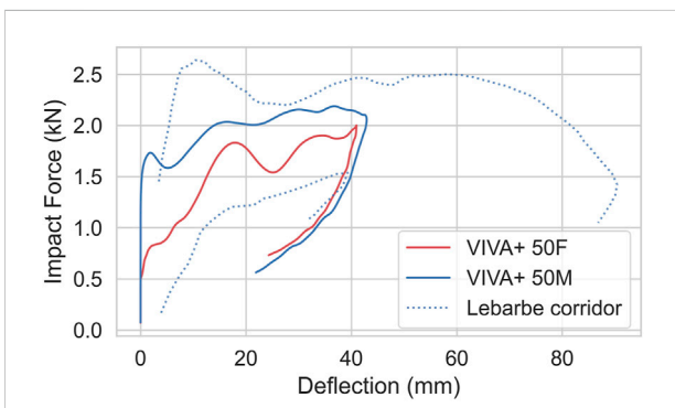
FIGURE 6 Blunt thorax impact simulations, compared to 4.3 m/s average male corridors from Lebarbé and Petit, 2012.
