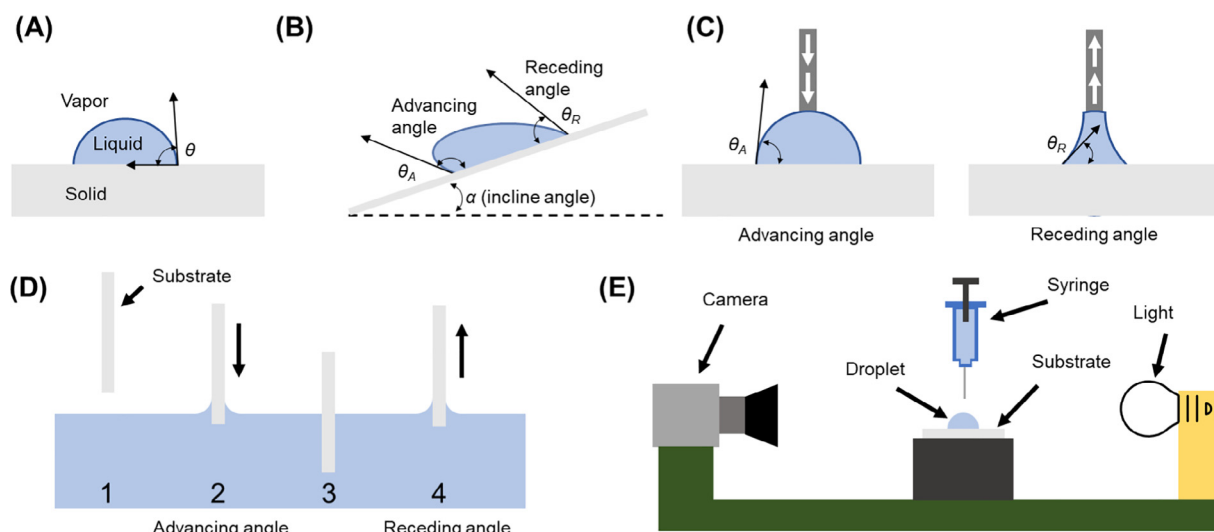
Fig. 1. A) Static contact angle. Schematics of setups of B) Tilting method, C) Needle method, and D) Wilhelmy plate method for the measurement of dynamic contact angle. E) A typical setup of a contact angle analyzer.
