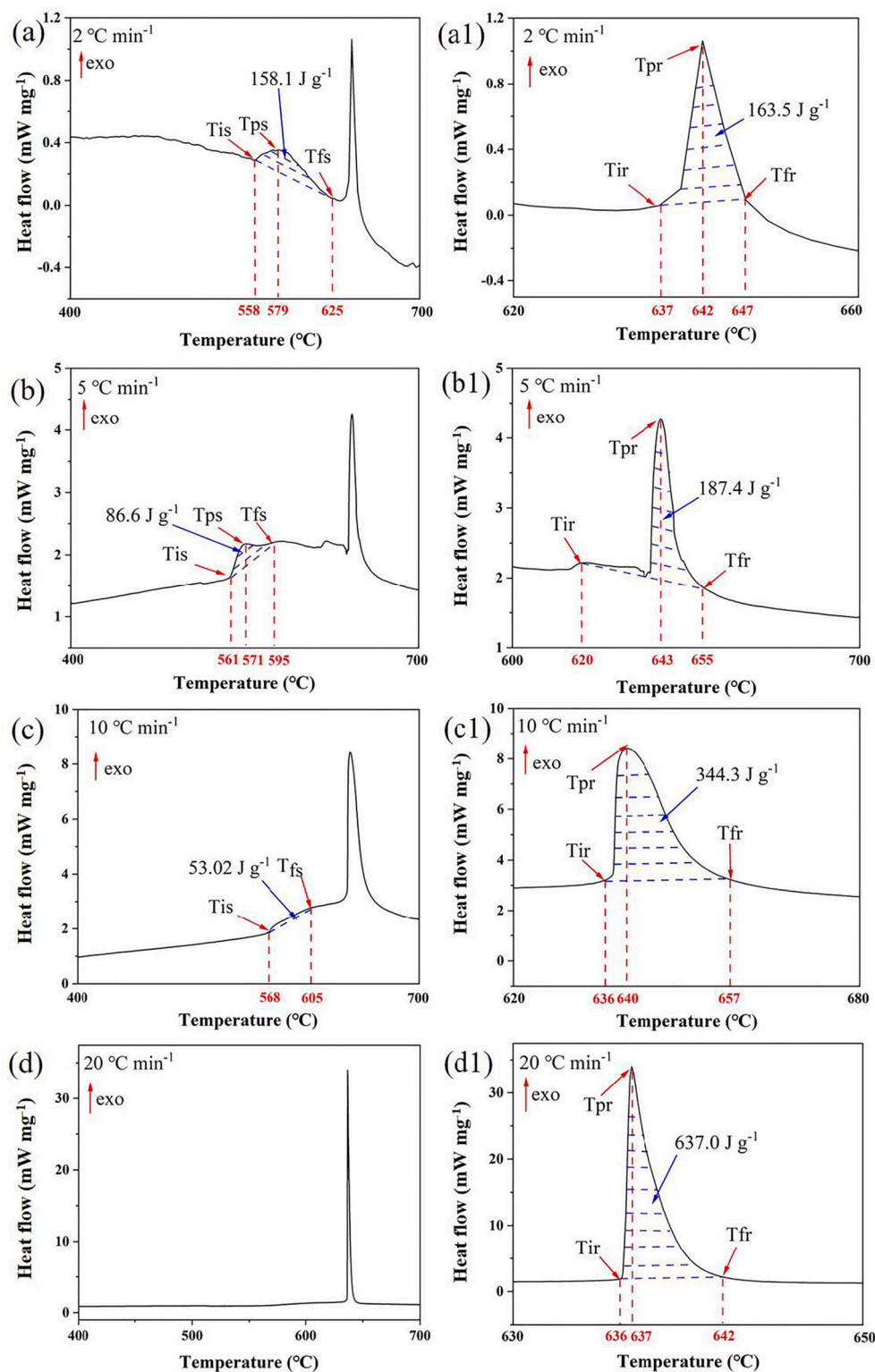
Fig. 3. DSC curves of porous NiAl at different heating rate: (a) 2\text{ }^{\circ}\text{C min}^{-1} , (b) 5\text{ }^{\circ}\text{C min}^{-1} , (c) 10\text{ }^{\circ}\text{C min}^{-1} and (d) 20\text{ }^{\circ}\text{C min}^{-1} . (a1)-(d1) corresponding zoom-in curves in the range of 600\text{--}700\text{ }^{\circ}\text{C} .
