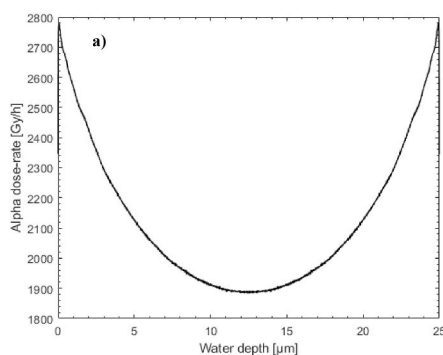
Fig. 11. \alpha dose rate in a 25 \mu\text{m} water depth crack (a) as well as the average \alpha dose rate over cracks with width 1\text{--}40 \mu\text{m} (b) together with an exponential fit, modelling the Tribet fuel with an \alpha -particle energy of 5.3 MeV, specific activity of 4.73\cdot 10^8 \text{ Bq}\cdot\text{g}^{-1} and a fuel density of 10.8 \text{ g cm}^{-3} .
