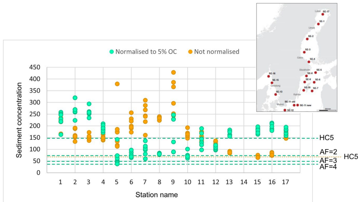
Figure 3: Surface sediment concentrations at Swedish marine stations (see map) from 2014. The green dots represent the normalised data (to 5% OC) while the orange dots are not normalised. The dashed green lines show the level of HC5-50 and the EQS values applying an assessment factor of 2, 3 and 4. The yellow dashed line show the HC5-50 value from an SSD analysis conducted on non-normalised data.
