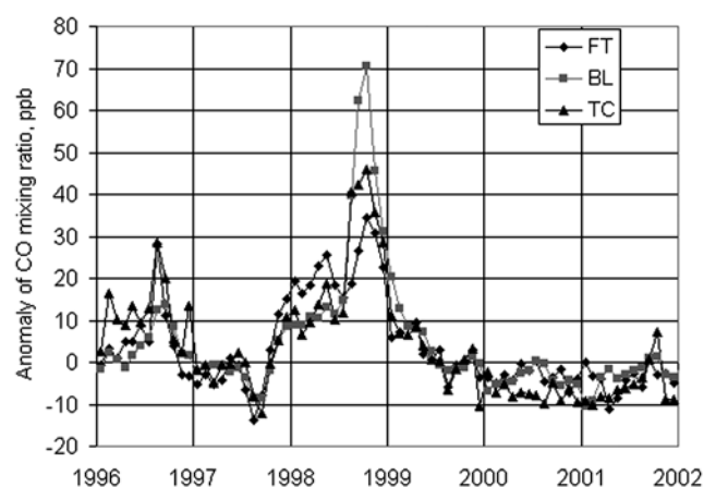
Figure 5. Average anomalies for three atmospheric domains expressed in parts per billion. Free troposphere (FT) includes data for all the mountain stations, both in situ and total column. Boundary layer (BL) comprises the low level in situ data. Total column (TC) is the average of the data for five low-level total column stations (total column amounts of CO were divided by the total numbers of air molecules). See color version of this figure in the HTML.
