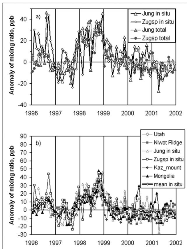
Figure 4. Monthly mean CO anomalies for high-altitude stations (with altitudes higher than 900 m asl). (a) Jungfrauoch and Zugspitze; in situ and column amount anomalies are compared. Total column amounts were divided by the total numbers of air molecules for the layer between the altitude of the station and 10 km asl (according to the 1976 U.S. Standard Atmosphere). (b) Monthly mean anomalies of CO mixing ratio, measured in situ at the mountain stations (see Appendix A for the geographic coordinates and affiliations). See color version of this figure in the HTML.
