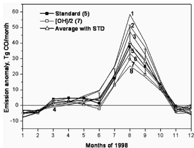
Figure 9. A study of the sensitivity of the calculated emission anomaly to the parameters of the box model. Full rectangles correspond to the standard set of parameters (M1, T1, and C1; see text); open rectangles are for the case that differs from the previous one by 2 times lower [OH] (options M1, T1, and C2). The numbers correspond to the combinations of parameters: 1 (M2, T1, and C1); 2 (M2, T2, and C1); 3 (M2, T1, and C2); 4 (M2, T2, and C2); 5 (M1, T1, and C1); 6 (M1, T2, and C1); 7 (M1, T1, and C2); 8 (M1, T2, and C2). See color version of this figure in the HTML.
