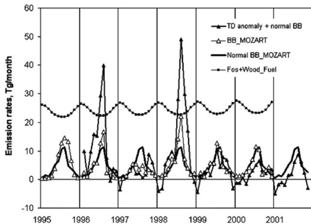
Figure 11. The top-down estimate for the biomass burning emission between 30°N and 90°N (full triangles) in assumption of normal emission rates from the MOZART inventory (solid line). BB is the inventory of biomass burning emission from boreal forest fires, other forest fires, and bush and savanna (steppe) fires. Fos +Wood_Fuel represents CO from combustion of coal, gas, and oil, and their products combined with CO from domestic wood fuel, used for heating and cooking. Normal BB is the average of biomass burning emissions over the period 1995–2000, except 1998. See color version of this figure in the HTML.
