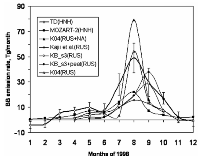
Figure 12. Comparison of the top-down (TD) estimate for CO emission from the biomass burning in 1998 with available inventories. HNH designates all biomass burning between 30°N and 90°N. “RUS” and “NA” correspond to emissions from boreal forest areas in Russia and North America, respectively. For definitions of inventories, see text. See color version of this figure in the HTML.
