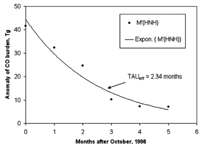
Figure 7. The exponential decay of CO anomaly after October 1998.
