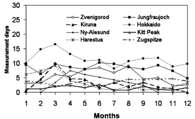
Figure A1. Numbers of measurement days per month averaged for 1996–2001. See color version of this figure in the HTML.
