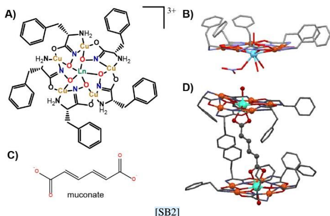
Scheme 1: Illustrations of (Ln^{III}[15-MC-Cu^{II}(L-pheHA)-5])^{3+} (A and B), [4a] dicarboxylate guest (C), and host-guest-host dimeric compartment (D). [4c]
