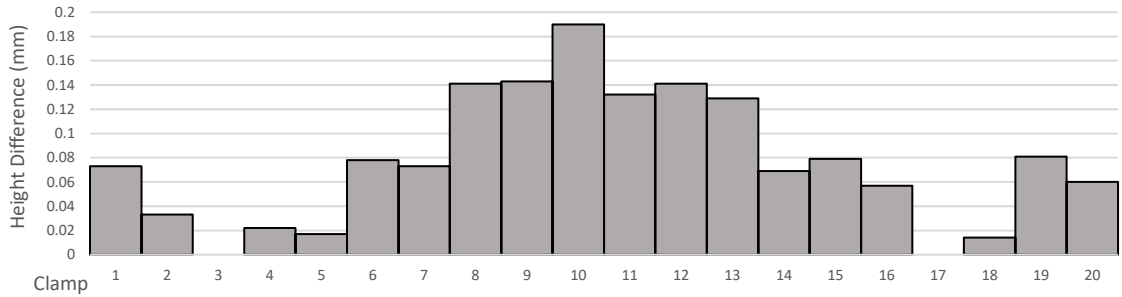
Fig. 8. Clamp heights.
