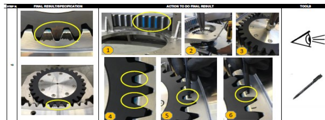
Fig. 3. SOP steps.
