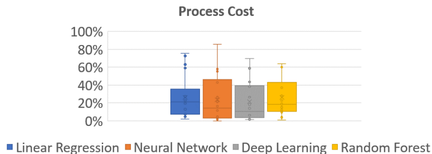
Figure 3.: MAPE for the different parametric cost modelling techniques (test 2).
