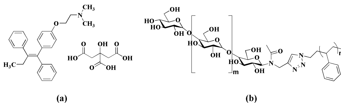
Figure 1. Chemical structures of (a) tamoxifen citrate and (b) maltoheptaose- b -polystyrene (MH- b -PS).
