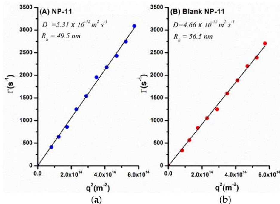
Figure 3. Dependence of relaxation frequency \Gamma ( s^{-1} ) on the square of wave vector modulus ( q^2 ) for (a) NP-11 and (b) blank NP-11.
