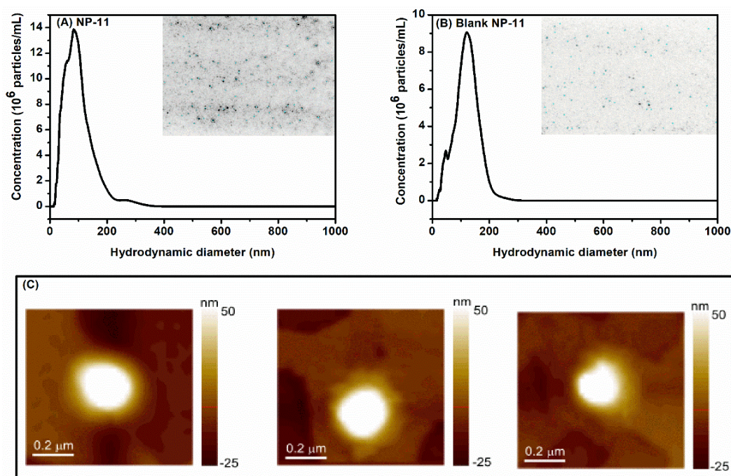
Figure 4. Size distribution for (A) NP-11 and (B) blank NP-11 from NTA measurements. Inserts show NTA video frames for both samples. (C) AFM images obtained for NP-11.
