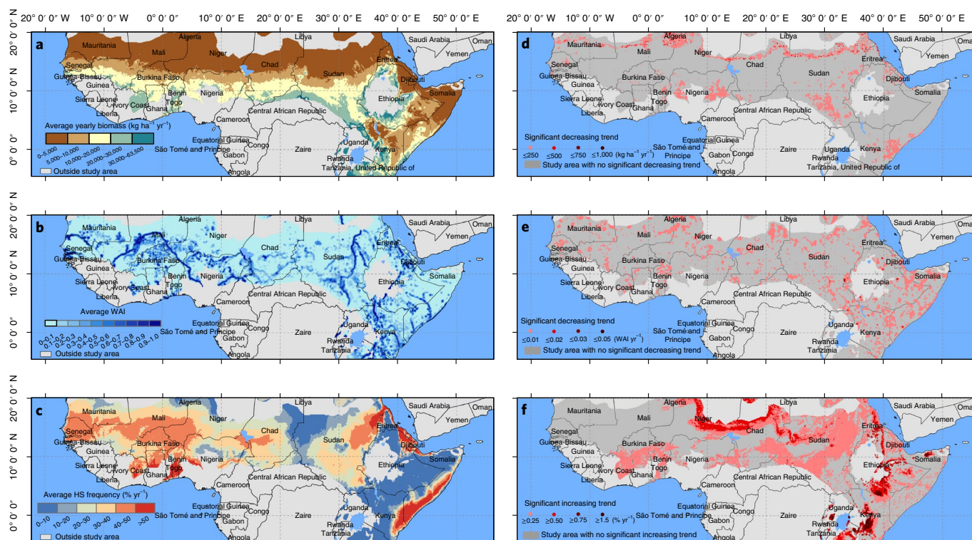
Fig. 1 | Averages and regional trends of DMP, WAI and HS. a–c , Long-term average annual DMP ( a ), WAI ( b ) and HS ( c ). d–f , Regional significant trends ( P \leq 0.05 ) in DMP ( d ), WAI ( e ) and HS ( f ) over the past two decades (2001–2020).
