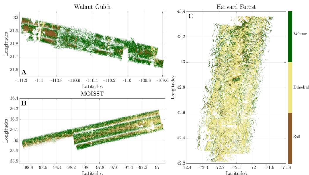
Figure 5. Estimated normalized, relative power indices representing dominant soil ( P_s/P_t ), dihedral ( P_d/P_t ), or volume ( P_v/P_t ) scattering at the AirMOSS monitoring sites. The average values of the most dominant scattering mechanism of all dates are displayed (Figure 1, Section 2). White data gaps originate from initial filtering of the input parameters. (A) Walnut Gulch, AZ, USA. (B) MOISST, OK, USA. (C) Harvard Forest, MA, USA.
