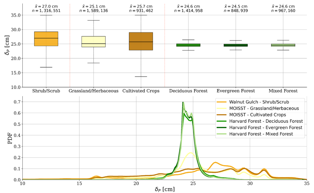
Figure 9. Boxplots and probability density functions (PDFs) of estimated permittivity-based penetration depths \delta\rho for main land cover classes at the AirMOSS monitoring sites Walnut Gulch, MOISST, and Harvard Forest. The results are displayed for all acquisition dates (Figure 1, Section 2). \bar{x} represents the respective median value, n is the total amount of values per boxplot.
