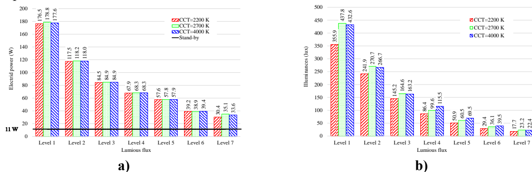
Figure 3. Characterisation of the whole lighting system: (a) electric power required and (b) illuminance values on the task area (sensor H2).
