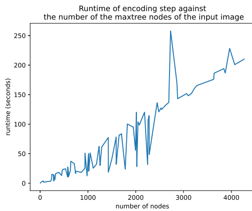
Fig. 20. Runtime experiment plot.
