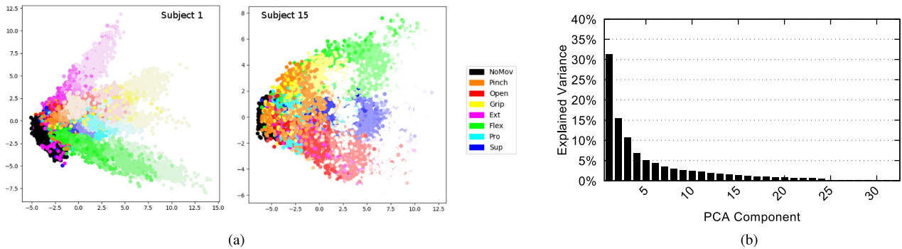
Fig. 5. Analysis of the feature space, using standard Hudgins features. (a) Scatter plot of features in PCA space (two most relevant components), for a typical subject (#1) and a badly performing subject (#15). Lighter color means greater contraction strength. (b) Explained variance per PCA component on features from all movements, averaged over development subjects.
