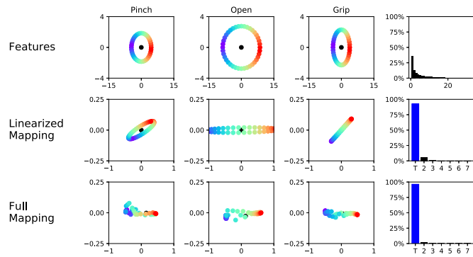
Fig. 8. Linearized mapping of diverse movements of subject 7 in PCA space, for the reference neural network. Right column shows explained variances averaged over all movements.
