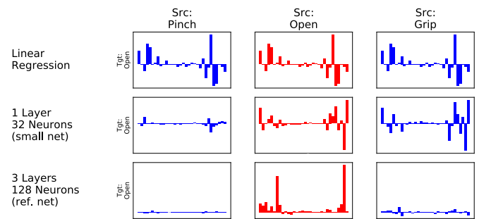
Fig. 7. Linearization of the mapping for the target movement Hand Open in different regions, for several regressors. Each panel shows the linearization of the mapping as a 32-dimensional weight vector in feature space, each column refers to the region of the features for a specific source movement.
