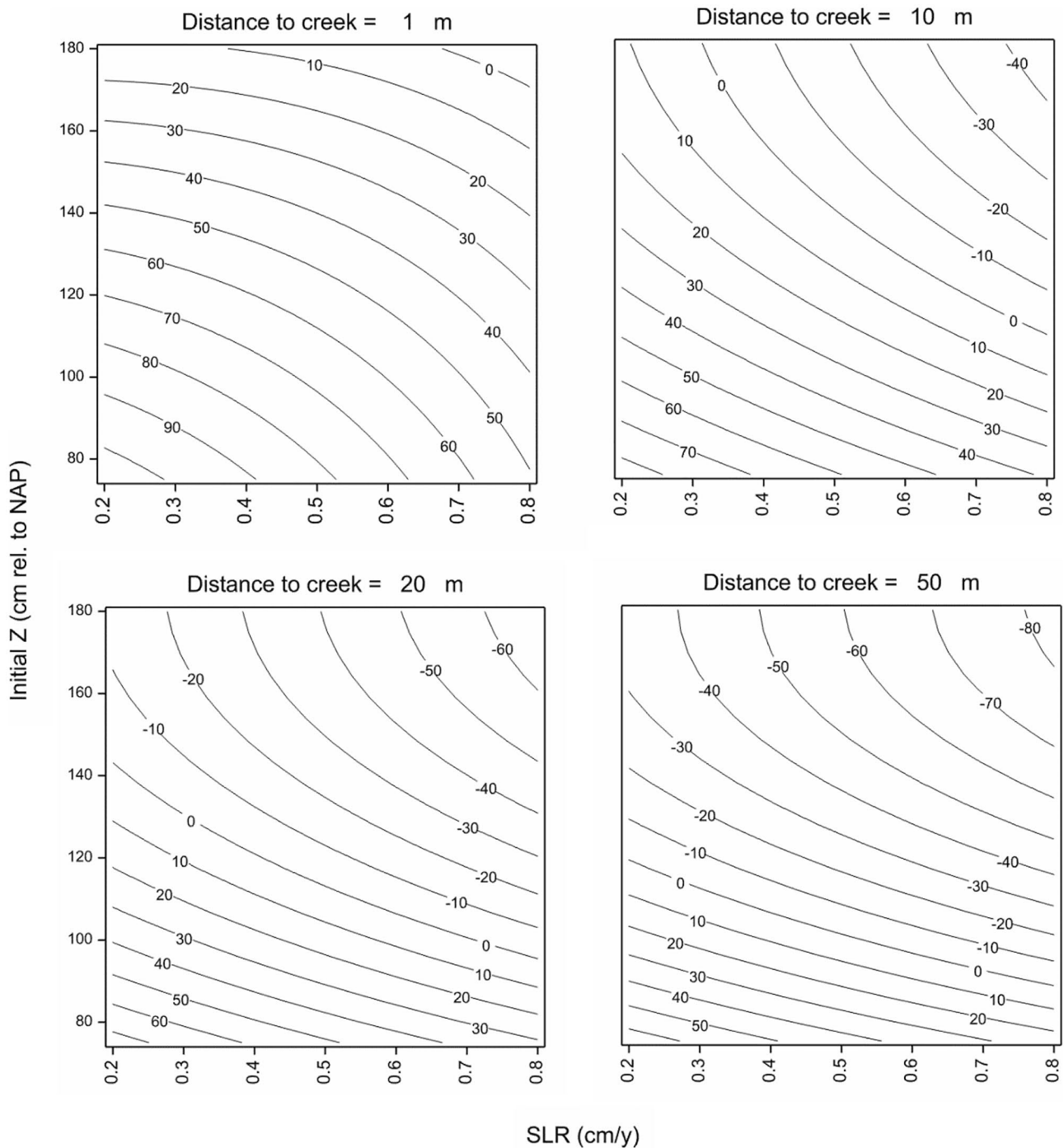
Fig. 7 Contour plots of predicted accretion surplus (=surface elevation change in cm relative to sea level) after 100 years as a function of initial elevation ( Z ) and rate of SLR, at various distances to the nearest creek. Simulated values resulting from the model with the highest
