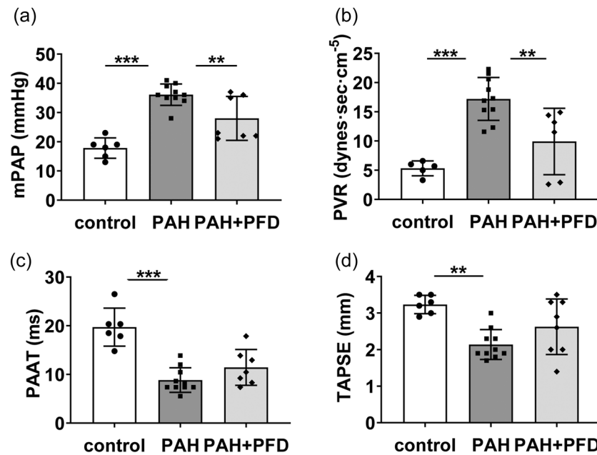
FIGURE 1 Effects of pirfenidone (PFD) on hemodynamics in the monocrotaline and aortocaval shunt rat model for PAH: PAH was induced in rats by intraperitoneal injection of 1 ml (60 mg/ml) monocrotaline followed by aortocaval shunt surgery 7 days later. Controls received injections with saline and underwent sham surgery. PAH animals were randomly divided into two groups: the PAH and PAH+PFD groups. The PAH group received a chow diet. The PAH+PFD group received a chow diet supplemented with 0.4% PFD. Hemodynamics were assessed 20 days after aortocaval shunt surgery. (a) mPAP: mean pulmonary arterial pressure; (b) PVR: pulmonary vascular resistance; (c) PAAT: pulmonary artery acceleration time; and (d) TAPSE: tricuspid annular plane systolic excursion. * p < 0.05 ; ** p < 0.01 ; *** p < 0.001 by two-sided one-way ANOVA with Holm–Sidak’s post hoc correction. ANOVA, analysis of variance; PAH, pulmonary arterial hypertension.
