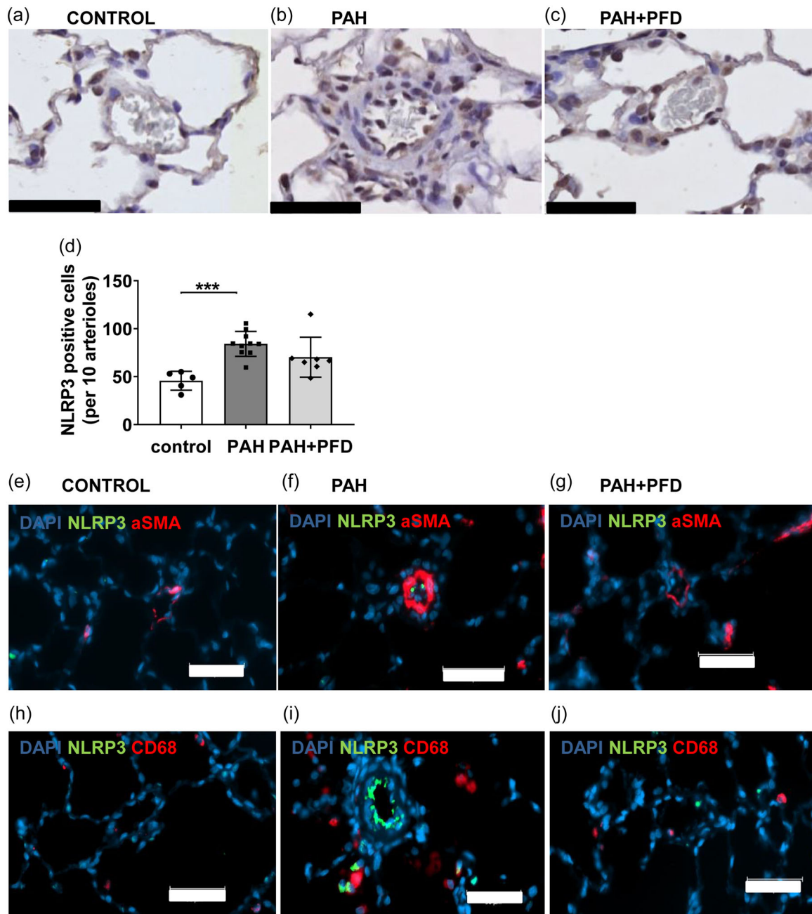
FIGURE 3 PAH induces NLRP3 expression in the distal pulmonary bed: Paraffin sections from lungs were stained for NLRP3. (a–c) Representative pictures of pulmonary arterioles stained for NLRP3 (dark brown); (d) number of NLRP3 positive cells per 10 pulmonary arterioles; (e–g) representative arterioles of double stainings of NLRP3 (green) and \alpha -smooth muscle actin ( \alpha -SMA) in red; and (h–j) representative arterioles of double stainings of NLRP3 in green and CD-68 in red; scale bar = 50 \mu m; *** p < 0.001 by two-sided one-way ANOVA with Holm–Sidak’s post hoc correction. ANOVA, analysis of variance; DAPI, 4’,6-diamidino-2-phenylindole; PAH, pulmonary arterial hypertension; PFD, pirfenidone.
