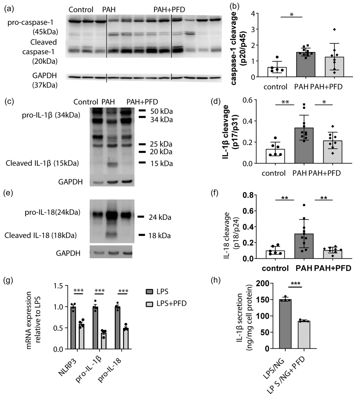
FIGURE 4 Effects of pirfenidone (PFD) on NLRP3 inflammasome activation in PAH lungs and in macrophages in vitro: Lung tissue was isolated from the rats as described in Figures 1–3, homogenized and cleavage of caspase-1 (a, b), IL-1 \beta (c, d), and IL-18 (e, f) were assessed by Western blot. Representative pictures are shown (a, c, e), and quantified (b, d, f). (g, h) Bone marrow was isolated from mice and differentiated into bone marrow-derived macrophages (BMDMs) in DMEM supplemented with a 20% L-cell conditioned medium for 7 days. Subsequently, BMDMs were treated with or without PFD (500 \mu\text{g}/\text{ml} ) o/n, and subsequently with lipopolysaccharide (LPS) (100 ng/ml) for 4 h. (g) Cells were lysed, RNA was isolated, and the expression of NLRP3, pro-IL-1 \beta , and pro-IL-18 mRNA was measured by qPCR and corrected for 36B4, cyclophilin B, and GAPDH (housekeeping genes). (h) Cells were subsequently treated with nigericin (NG) (20 \mu\text{M} ) for 30 min and IL-1 \beta secretion into the medium was assessed by ELISA and corrected for cell protein; * p < 0.05 ; ** p < 0.01 ; *** p < 0.001 by two-sided one-way ANOVA with Holm–Sidak’s post hoc correction. ANOVA, analysis of variance; ELISA, enzyme-linked immunosorbent assay; IL-1 \beta , interleukin-1 \beta ; mRNA, messenger RNA; PAH, pulmonary arterial hypertension; qPCR, quantitative polymerase chain reaction.
