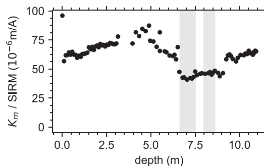
Figure 9. Depth profile of K_m / \text{SIRM} . Shaded areas indicate the intervals with the inverse AMS fabrics (6.65–7.5 and 8–8.6 m).
