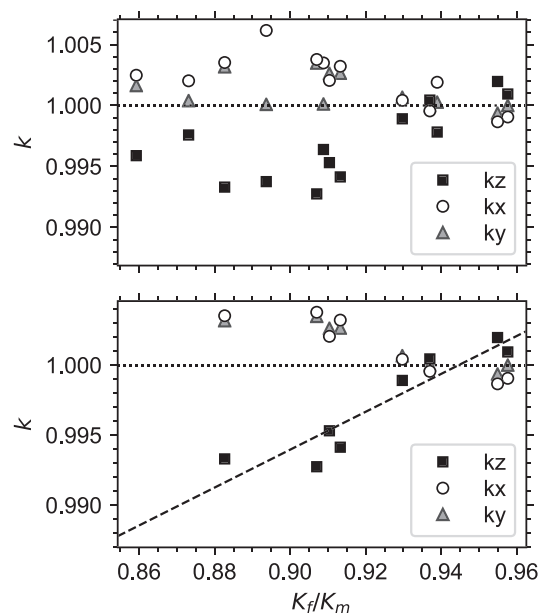
Figure 11. Normalized principal AMS versus K_f/K_m . Solid squares represent k_z , open circles k_x , and gray triangles k_y . (top) Data spanning the entire core. (bottom) Data for samples below 5.5 m. Horizontal dotted line shows k = 1 . Dashed line in the bottom plot is a linear fit to k_z .
