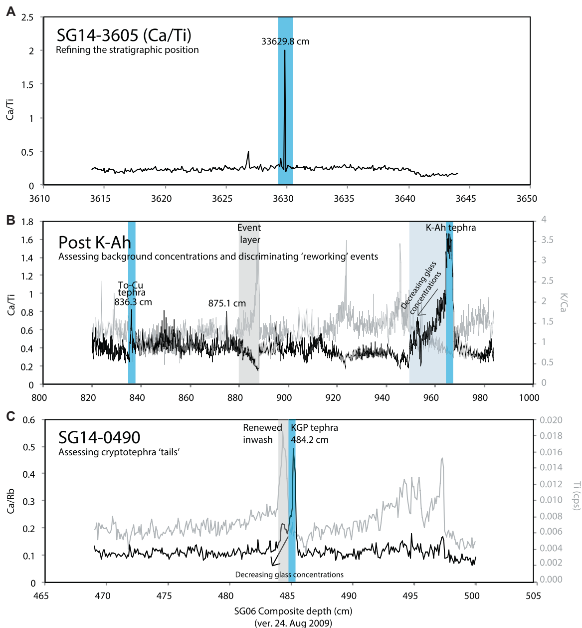
Figure 4. Selected \mu XRF elemental profiles over the positioning of several key visible and cryptotephra layers preserved in the Lake Suigetsu sediments. These examples highlight the ability of \mu XRF to assist in the identification and interpretation of the glass concentrations by: (a) refining the precision of the stratigraphic position of the peak; (b) the ability to identify primary cryptotephra layers during periods of high background glass concentrations (>5000 shard per gram), i.e. the To-Cu tephra at 836.3 cm CD (the compositional spike at 875.1 cm CD was investigated and it does not correspond to a tephra layer); and (c) the opportunity to track cryptotephra tails, renewed inwash events (using Ti) and determine the initial input/eruption position. The blue shading shows the position of the cryptotephra as determined by density separation techniques where the resolution is 1 cm. The grey bars show the position of crypto-event layers defined using the \mu XRF elemental responses shown. [Color figure can be viewed at wileyonlinelibrary.com ]
