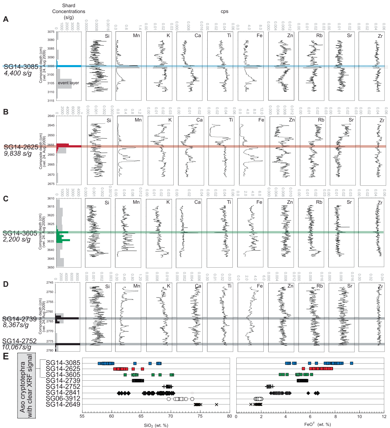
Figure 5. (a–d) Comparison of the glass shard concentrations (in shards per gram of dry sediment) and elemental profiles for Si, Mn, K, Ca, Ti, Fe, Zn, Rb, Sr and Zr (in cps normalised to incoherent plus coherent) across the known cryptotephra layers that have been correlated to eruptions of Aso (SG14-3085, SG14-2625, SG14-3605, SG14-2739 and SG14-2752). The cryptotephra counts are from McLean et al. (2020b). Horizontal lines indicate the positioning of the cryptotephra peak as determined using density separation techniques. (e) Glass compositions of the visible (e.g. SG06-3912) and cryptotephra layers erupted from Aso caldera and preserved in the Lake Suigetsu sediments between 50 and 30 ka (from McLean et al. , 2020b). [Color figure can be viewed at wileyonlinelibrary.com ]
