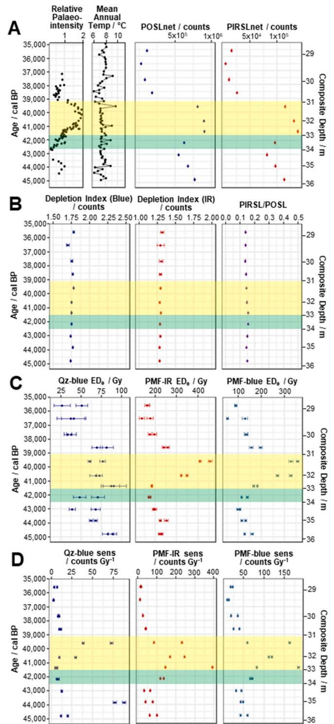
Fig. 2. Results of the POSL (Panels A and B) and lab profiling (Panels C and D) analysis for the 11 samples in Time Period 2. Panel A also shows contextual data (relative palaeointensity ( J_{200^\circ\text{C}}/J_{200^\circ\text{C}} ; Hyodo et al., 2022) and pollen-reconstructed mean annual temperature from Suigetsu). Green horizontal bars highlight the Laschamp geomagnetic excursion. Yellow horizontal bars highlight the period of higher relative palaeointensity following the Laschamp.
