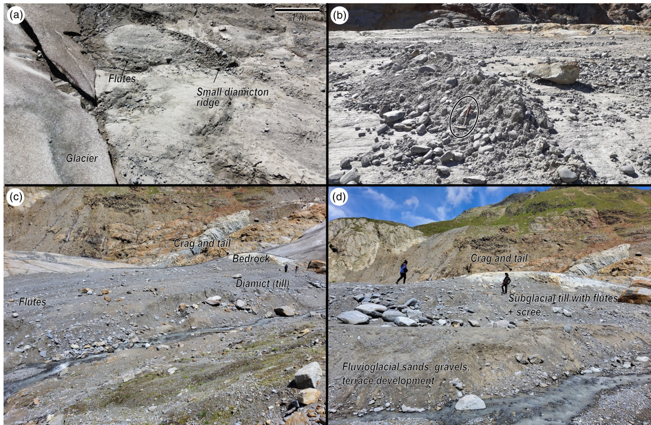
Fig. 4. Images of the subglacial sediment–landform assemblage. (a) Aerial view of the glacier margin and its immediate forefield, showing a glacier-margin parallel crevasse and a small annual moraine in the forefield. (b) Detail of the annual moraine, which consists largely of subglacial diamictons with a surface veneer of angular, supraglacial debris. In the background, flow parallel flutes and a low profile crag and tail structure can be seen imaged in (c) and (d). Looking south. (c, d) Images of a till blanket, moulded into flutes, and a crag and tail structure. Both images taken looking NE, with photo (c) somewhat further from the ice margin. All photographs (a–d) taken in July 2020.
