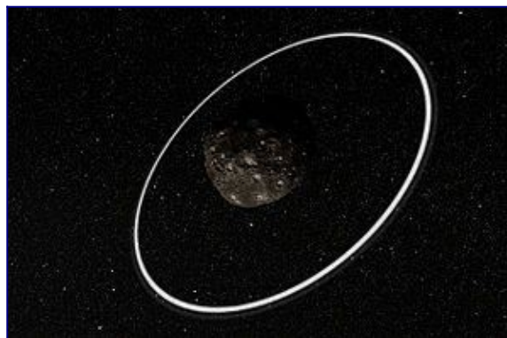
asteroid 10199 Chariklo with Ringsystem – artistic rendering
