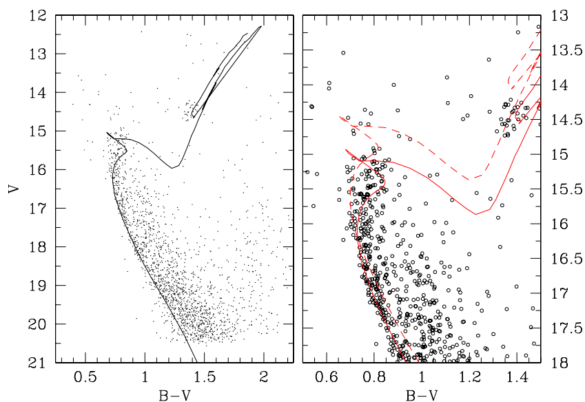
Figure 8. Left panel: isochrone fitting to Trumpler 20 CMD for the set of parameters discussed in Section 7, namely, 0.35 mag, 13.7 mag, and 1.4 Gyr for reddening, distance modulus, and age, respectively. Right panel: a zoom of the TO region. The solid line is the same isochrone as in the left panel, while the dashed one is again the same isochrone but shifted by 0.7 mag to account for unresolved binary stars.
