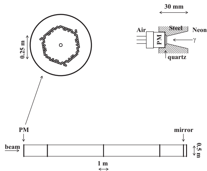
Fig. 1. The RICH prototype setup. At the bottom a side view of the prototype is shown; a front view of the upstream endcap is shown on the top left; a detail of the upstream endcap cut, together with a photomultiplier, is shown on the top right. The scales are different in each picture, as indicated; in the bottom plot the horizontal and vertical scales are also different.
