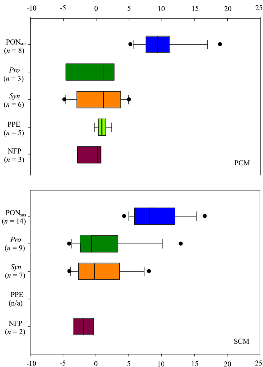
Fig. 3. Boxplot of the \delta^{15}\text{N} natural abundance from PON sus (0.3–3.0 \mu\text{m} size fraction) and the \delta^{15}\text{N} of sorted picoplankton components from the PCM (top panel) and SCM (bottom panel); Prochlorococcus ( Pro ) and Synechococcus -like ( Syn ), PPE, and NFP. n is the number of measurements per group and n/a indicates that data were not available.
