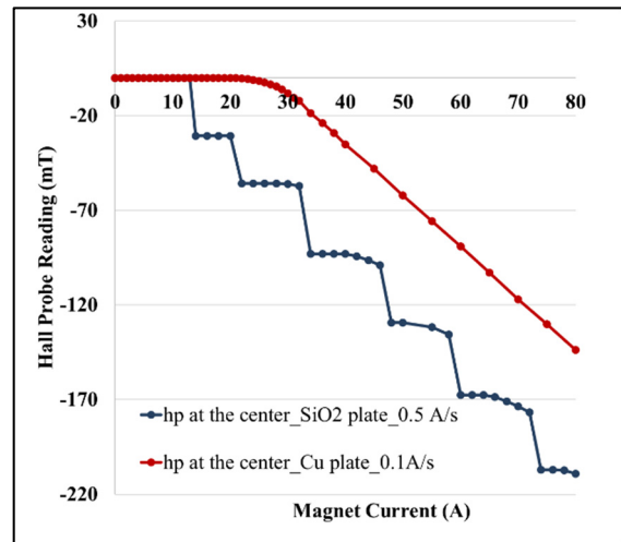
Figure 8: The measurement of \text{Nb}_3\text{Sn}/\text{Al}_2\text{O}_3 multilayers on \text{Al}_2\text{O}_3 wafer grown at University of Wisconsin [20].
