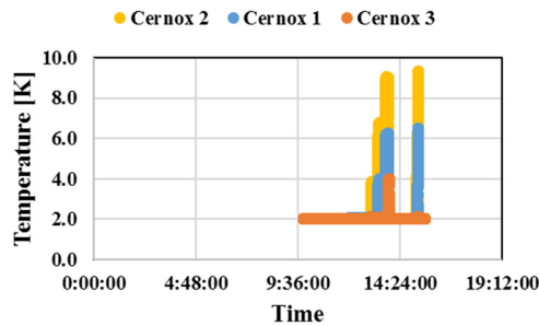
Figure 9: Measured temperature change in Cernox sensors.
