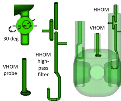
Figure 4: HHOM and VHOM couplers for the rf-dipole crabbing cavity.
