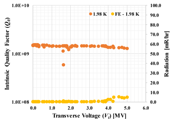
Figure 6: Q curve of the RFD-CAV-002 with both HHOM and VHOM couplers (Test 1).
