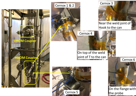
Figure 8: Locations of the Cernox sensors on the HHOM coupler.
