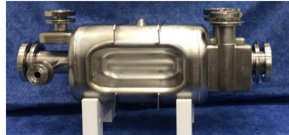
Figure 2: Fabricated Nb rf-dipole cavity.
