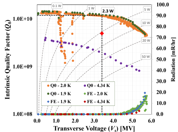
Figure 3: Q curves of the bare RFD-CAV-002.
