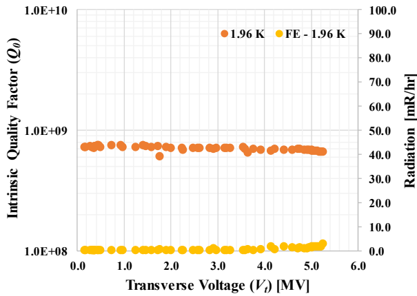
Figure 7: Q curve of the RFD-CAV-002 with only HHOM coupler (Test 2).
