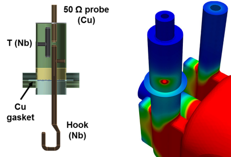
Figure 10: Cu gasket location at the HHOM coupler (left) and rf losses at the stainless steel flange (right).
