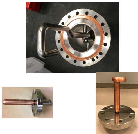
Figure 5: Nb HHOM high pass filter with hook and T (top), HHOM coupler probe (bottom left) and VHOM coupler (bottom right).
