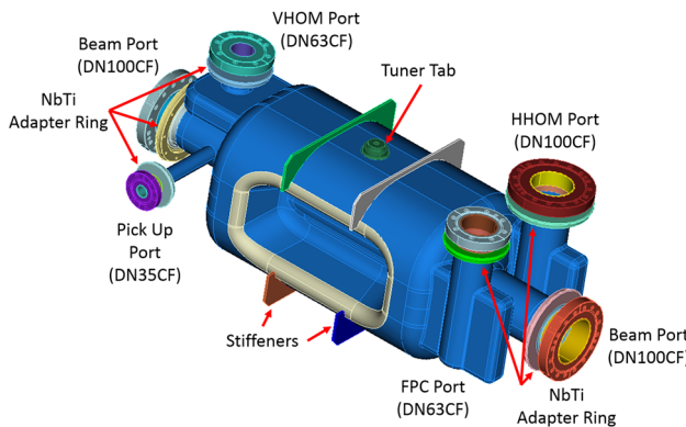
Figure 1: 400 MHz SPS prototype rf-dipole cavity.
