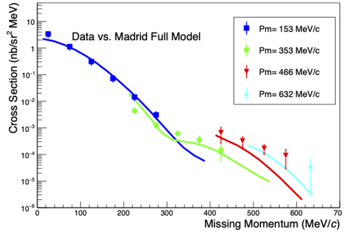
FIG. 9. E08009 data compared to Madrid full theoretical calculations. Blue squares are for the 153 MeV/c setting, green circles are for the 353 MeV/c setting, red inverted triangles are for the 466 MeV/c setting, and cyan triangles are for the 632 MeV/c setting. Theoretical calculations follow the same color code as the data for each momentum setting.
