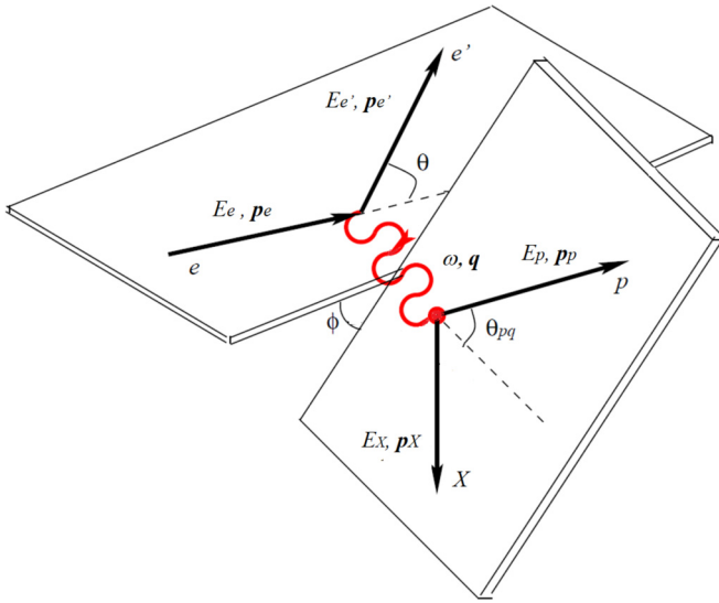
FIG. 1. Kinematic definitions for the A(e, e'p)X reaction.
