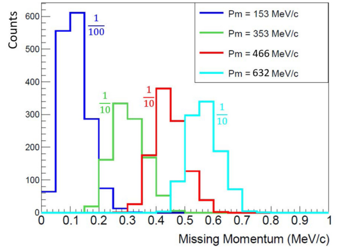
FIG. 3. Missing momentum spectra for all the kinematical settings of the experiment.
