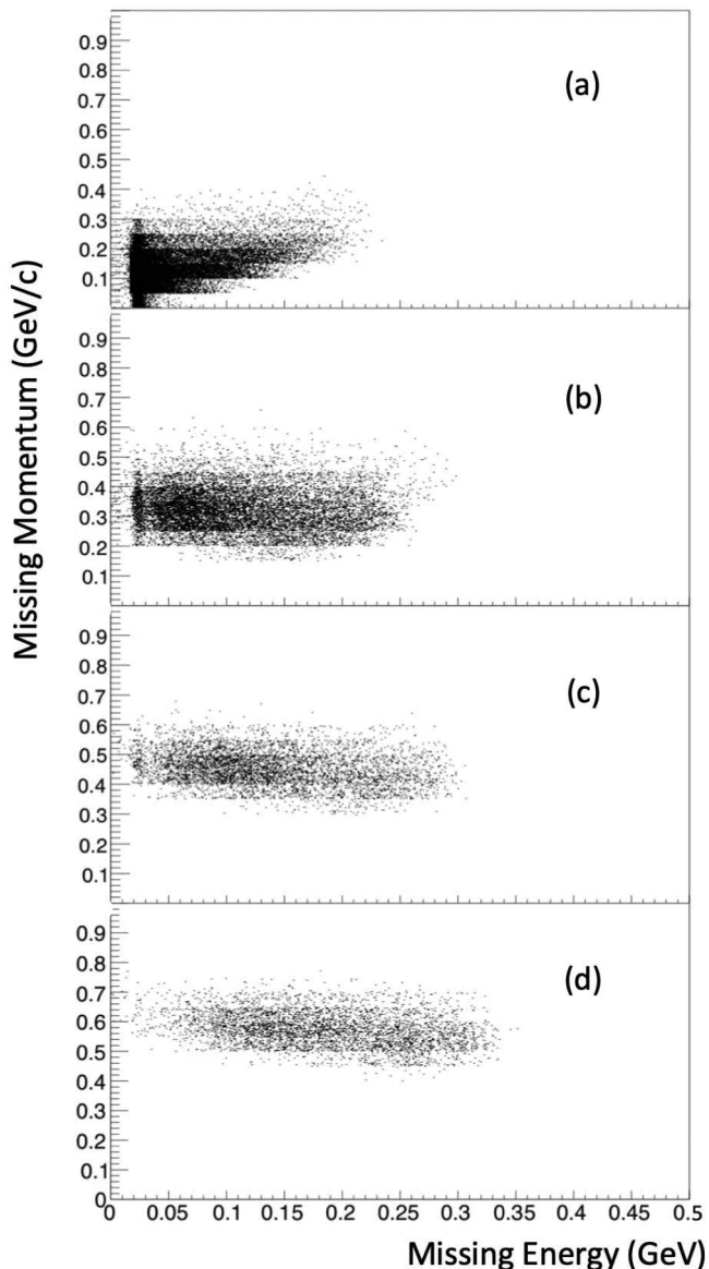
FIG. 6. Two-dimensional plots of missing momentum versus missing energy for the kinematical settings of the experiment. (a) p_m = 153 MeV/ c , (b) p_m = 353 MeV/ c , (c) p_m = 466 MeV/ c , and (d) p_m = 632 MeV/ c .
