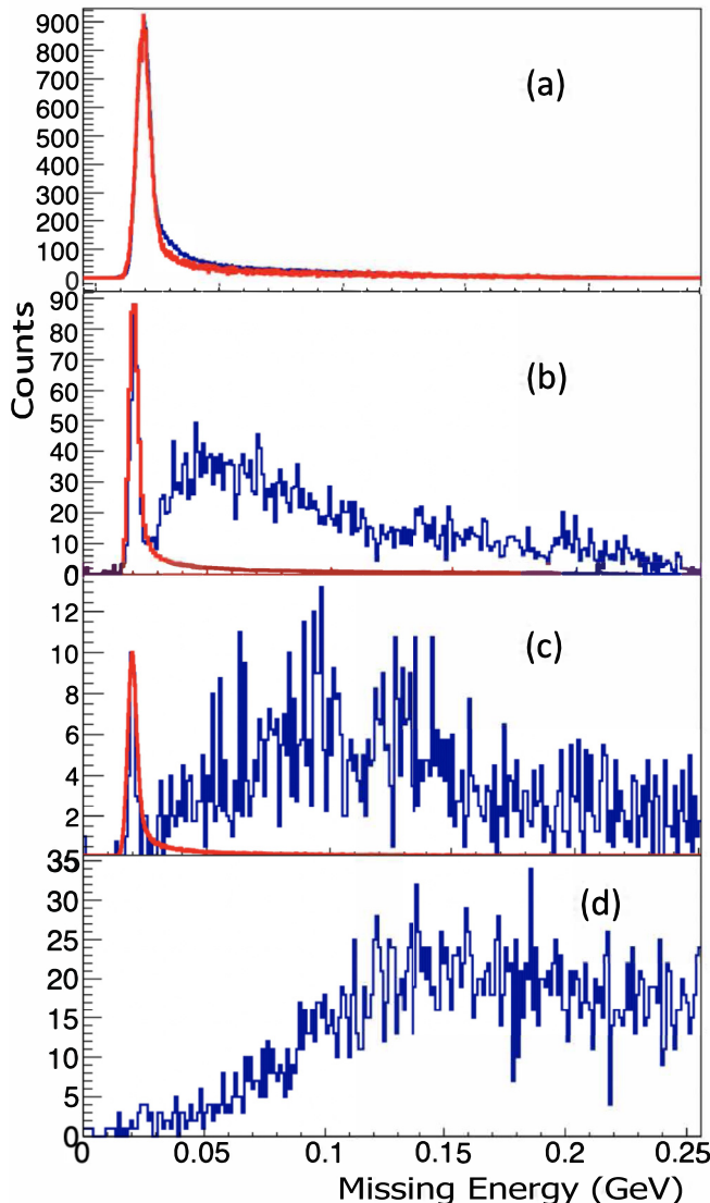
FIG. 5. Missing energy spectra for all the kinematical settings. Data are in blue and the simulated two-body breakup channel is in red. (a) p_m = 153 MeV/ c , (b) p_m = 353 MeV/ c , (c) p_m = 466 MeV/ c , and (d) p_m = 632 MeV/ c .
