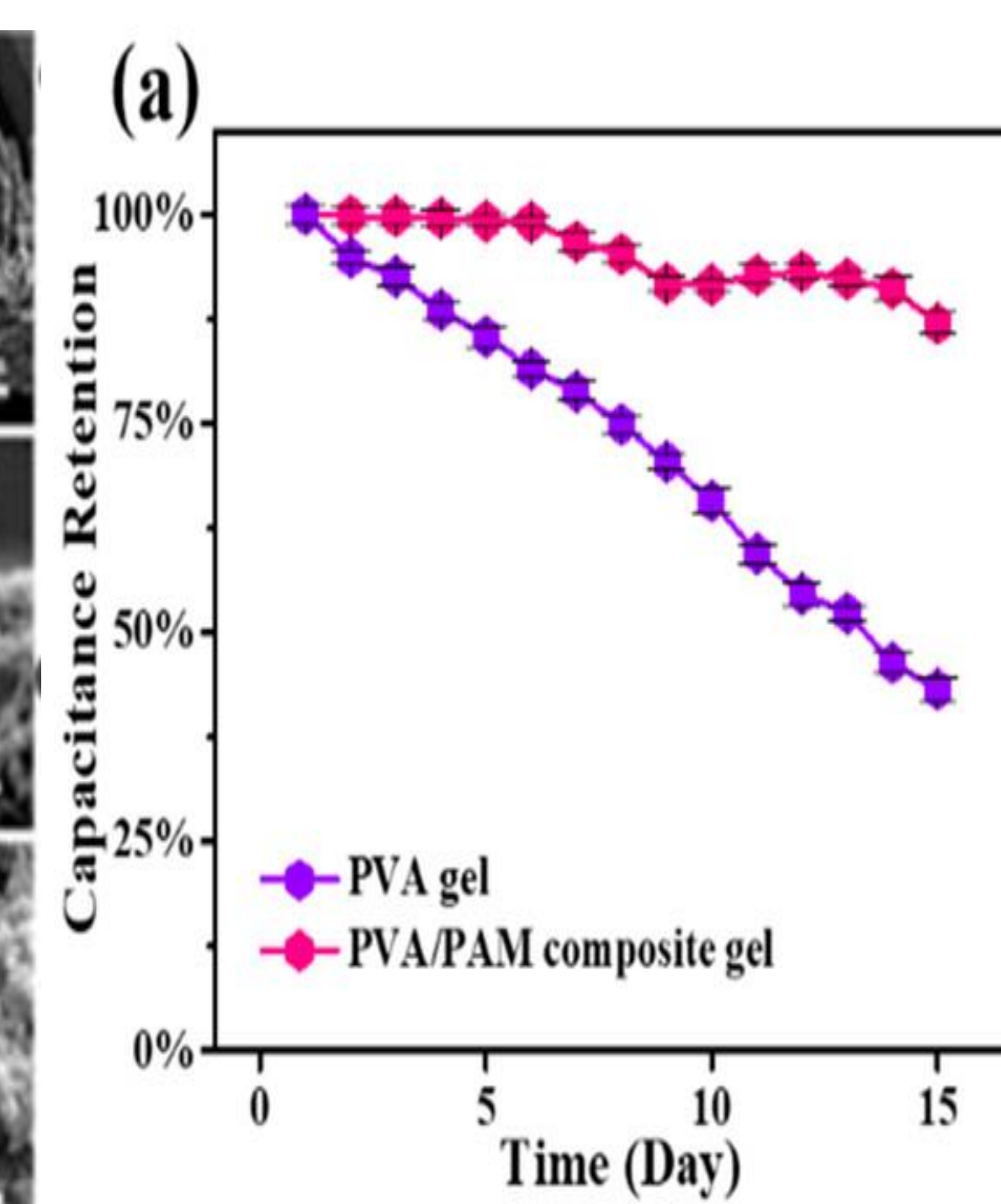
Fig 3: (a) Capacitance retention of G/PANI@HF-SCs based on PVA gel and PVA/PAM composite gel during 15 days, (b) water distribution in PVA gel and PVA/PAM composite gel, (c) the hydrogen bond between PVA and PAM molecule, (d) GCD curves of G/PANI@HF-SC in water for 1-12 h
