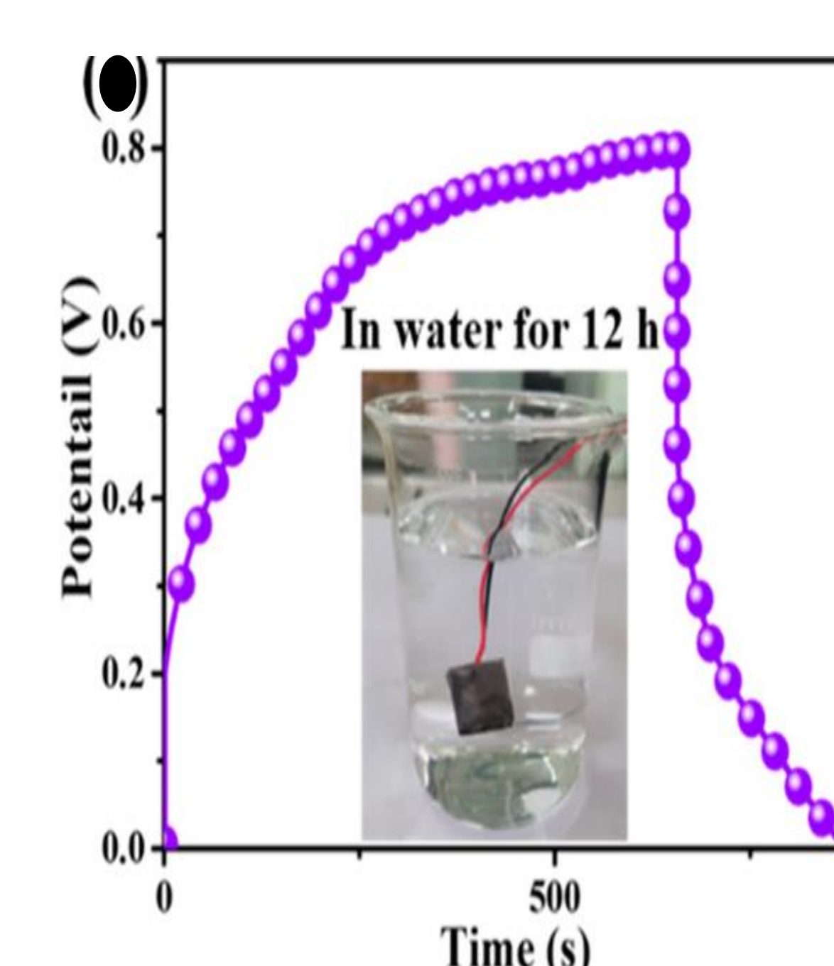
Fig 3: (a) Capacitance retention of G/PANI@HF-SCs based on PVA gel and PVA/PAM composite gel during 15 days, (b) water distribution in PVA gel and PVA/PAM composite gel, (c) the hydrogen bond between PVA and PAM molecule, (d) GCD curves of G/PANI@HF-SC in water for 1-12 h
