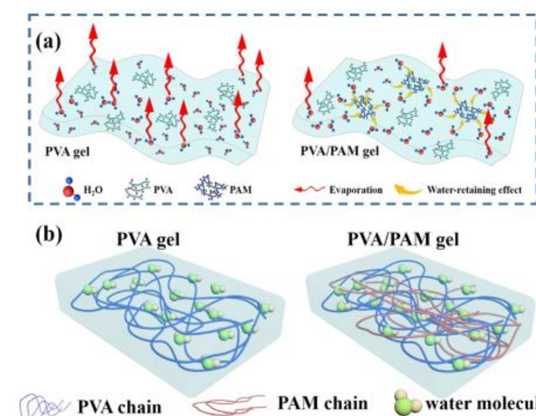
Fig 4: Schematic representation of the evaporation of water in gel electrolyte and water-retaining effect of PAM, and (b) crosslinked structure of PVA/PAM composite gel electrolyte.
