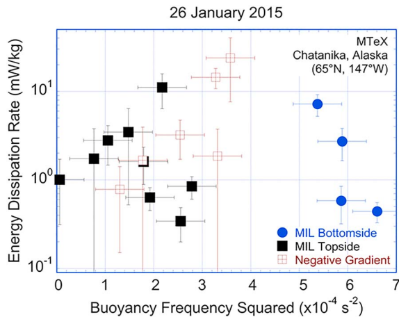
Figure 11. Turbulent energy dissipation rate plotted as a function of buoyancy frequency squared derived from MTeX CONE ion gauge measurements. The turbulent energy dissipation rates are separated based on either the presence of a MIL or the temperature gradient; on the bottomside of a MIL (blue circle), on the topside of a MIL (black square), and where the temperature gradient is negative above the MILs (red square with +). The error bars represent one-sigma statistical uncertainties in the measurements. MTeX = Mesosphere-Lower Thermosphere Turbulence Experiment; CONE = Combined Sensor for Neutrals and Electrons; MIL = mesospheric inversion layer.
