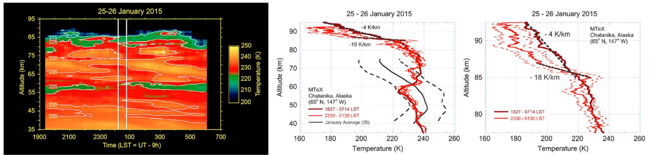
Figure 8. Temperature derived from Rayleigh lidar measurements at PFRR on the night of 25–26 January 2015 (LST). (left) Temperature plotted as a function of altitude and time. The two vertical white lines indicate the times when the MTeX payloads were launched (46.009 at 0013 LST, 46.010 at 0046 LST). (middle) Temperature plotted as function of altitude over full altitude range of lidar measurement. Average temperature profile for the whole night (1827–0714 LST, solid red), 2-hr profile spanning the MTeX launch period (2330–0130 LST, light red), one-sigma uncertainties in 2-hr profile (light red dashed), multiyear sample mean (solid gray), and standard-deviation profile (dashed gray). (right) Temperature plotted as function of altitude over subset of lidar measurement highlighting inversion layer and superadiabatic temperature gradient. The temperature gradients of -18 and -4 K/km are indicated on the temperature profiles. PFRR = Poker Flat Research Range; MTeX = Mesosphere-Lower Thermosphere Turbulence Experiment.
