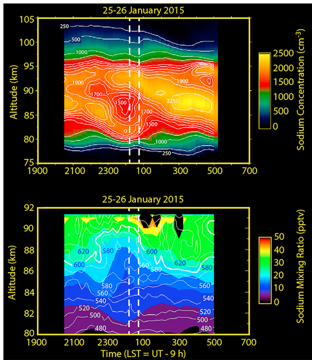
Figure 12. Sodium and potential temperature derived from resonance and Rayleigh lidar measurements at PFRR on the night of 25–26 January 2015. (top) Sodium concentration as a function of altitude and time. The two vertical lines mark the times when the MTeX payloads were launched (46.009 at 0013 LST, 46.010 at 0046 LST). The contours are 250, 500, 1,000, 1,250, 1,500, 1,600, 1,700, 1,800, 1,900, 2,000, 2,250 \text{cm}^{-3} . (bottom) Sodium mixing ratio (false color) and potential temperature (white contour). The potential temperature is calculated starting at 61 km, and thus, the values of potential temperature are lower than if calculated from the ground level. The 600-K contour is plotted bold. The potential temperature contour labels are plotted white and blue for clarity. The two vertical dashed lines mark the times when the MTeX payloads were launched. PFRR = Poker Flat Research Range; MTeX = Mesosphere-Lower Thermosphere Turbulence Experiment.
