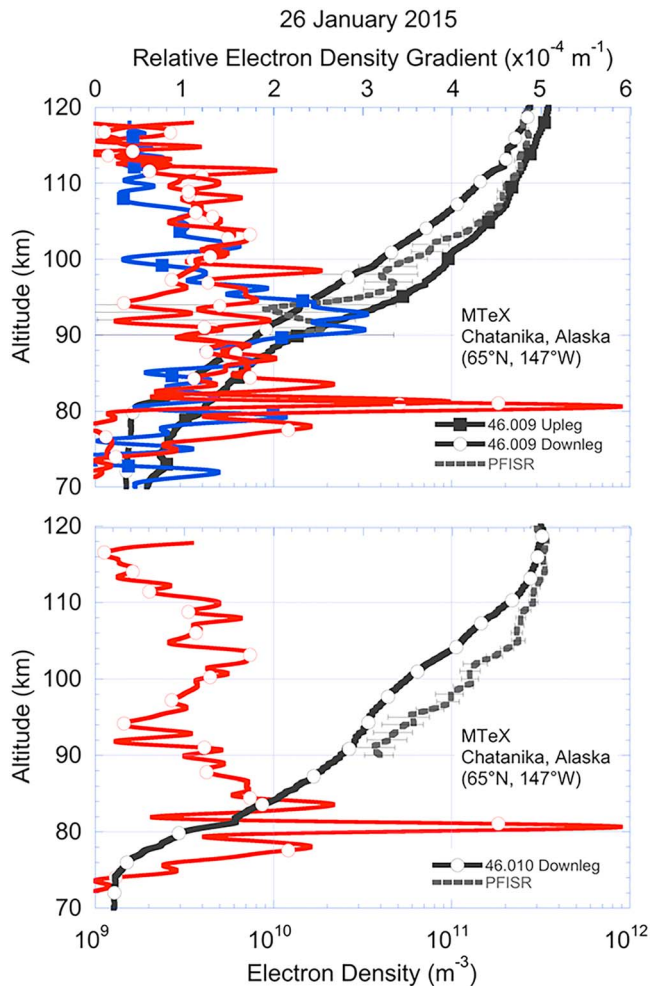
Figure 7. Electron density (black) and relative electron density gradients (blue and red) plotted as a function of altitude for 46.009 (top) and 46.010 (bottom) payloads. The rocket measurements are plotted in solid for upleg (closed square) and downleg (open circle). The PFISR measurements are plotted as a gray dashed line. The uncertainty in the Langmuir probe measurements is 2 \times 10^8 \text{ m}^{-3} in the electron density. The PFISR profiles are plotted with one-sigma error bars. PFISR = Poker Flat Incoherent Scatter Radar.
