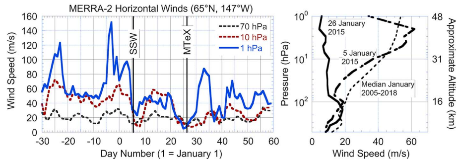
Figure 5. MERRA-2 horizontal wind speeds over Chatanika. (left) Daily horizontal wind speed over Chatanika at 70 (~18 km, gray dashed), 10 (~31 km, red dashed), and 1 hPa (~48 km, blue solid) plotted against UT day from December 2014 to February 2015. Winds are taken at 0600 UT each day. The black vertical lines mark the dates when the SSW split the stratospheric vortex (SSW, 5 January 2015) and the MTeX launch (MTeX, 26 January 2015). (right) Vertical profile of horizontal wind on 5 January (short-long dash), 26 January (solid), and median for January 2005–2018 (short dash) plotted as a function of pressure. The corresponding approximate altitude is given on the right axis. MERRA-2 = Modern-Era Retrospective Analysis for Research and Applications version 2; SSW = Sudden Stratospheric Warming; MTeX = Mesosphere-Lower Thermosphere Turbulence Experiment.
