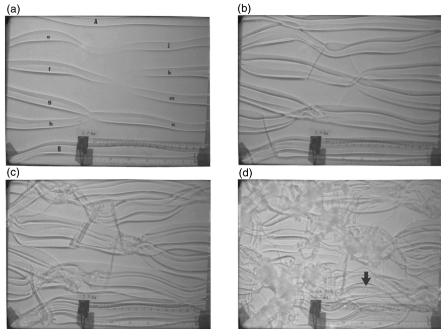
Figure 13. Four-panel images. The panels are based on Figure 2 from Thorpe (2002). The arrow in Panel (d) is from Thorpe (2002) and points to apparent convective rolls in the laboratory data similar to those in the atmosphere indicated by the light green arrow in Figure 5.
