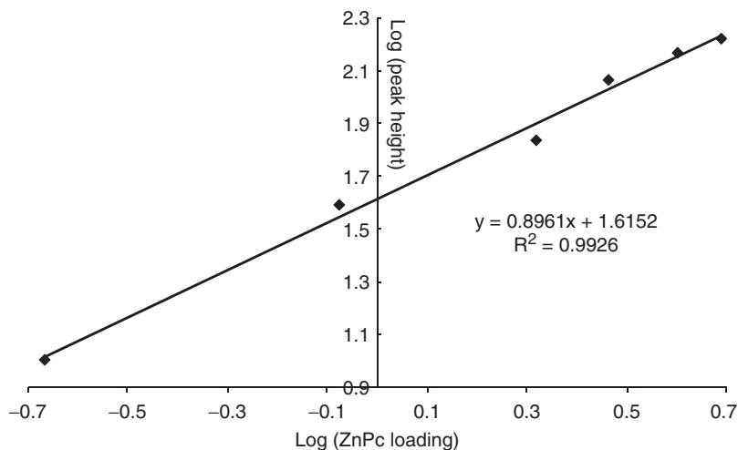
Figure 6. Plot of log (peak height) vs. log ZnPc loading to determine the reaction order with respect to ZnPc.
