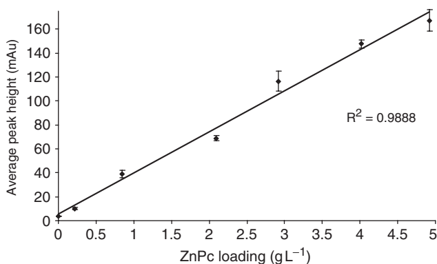
Figure 5. Plot of relative peak height vs. ZnPc loading to determine the effect of ZnPc on the phototransformation of 4-Np to fumaric acid ([4-Np] = 1 \times 10^{-5} mol dm -3 , pH = 9).
