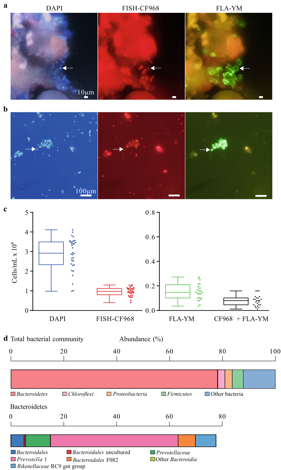
Fig. 1 YM utilization by Bt Bov isolates. Images of a 100 \mu\text{m} on food particles and b 10 \mu\text{m} filtered rumen extract incubated with FLA-YM and stained with DAPI and Bacteroides -FISH probe (FISH-CF968). Cells were visualized by epifluorescence microscopy. c Counts of cells from FLA-YM incubated rumen extract stained with DAPI, FISH-CF968, FLA-YM, and both FISH-CF968 and FLA-YM. Mean \pm standard deviation shown. d 16S rRNA metagenomics sequencing data of extracted rumen communities showing most prevalent phyla (left) and the distribution of Bacteroidetes spp. (right). N = 4
