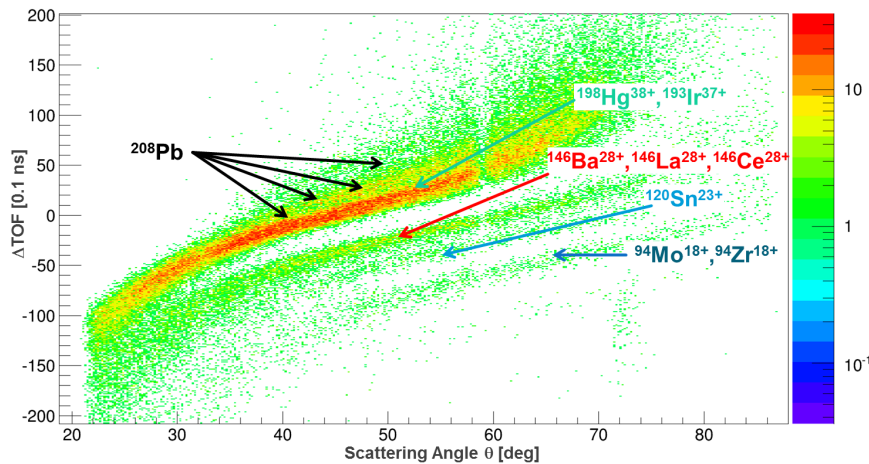
Figure 1: TOF vs. scattering angle recorded by CHICO2 in coincidence with a \gamma ray recorded in GRETINA. The A=146 group is easily distinguished from the stable beam contaminants.
