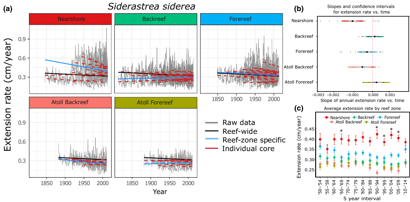
FIGURE 2 (a) Results of linear model of extension rate (cm/year) versus time for Siderastrea siderea by reef environment for the 1814–present interval. Gray lines are raw extension data, black lines are average linear models of extension for all S. siderea cores across all reef environments, blue lines are average linear models of extension for all S. siderea cores within each reef environment, and red lines are linear models of extension for individual S. siderea cores within reef environments. Raw (gray) and linearly modeled (red) extension chronologies highlight the variability in growth amongst colonies. (b) Slopes of linear models describe extension versus time for each reef environment, with small points representing individual cores and large points representing average slopes of all cores within a reef environment (gray bars and colored bars are 50% and 95% confidence intervals (CI), respectively, of average slope for each reef environment). Slopes are significantly different from each other if their 95% CI do not overlap. Likewise, slopes are significantly different from zero if their 95% CI do not overlap with the vertical red dashed line centered on zero. (c) Five-year averages of skeletal extension rate by reef environment \pm 1 SE. Asterisks indicate statistically significant differences ( p < .05 ) between nearshore and forereef values
