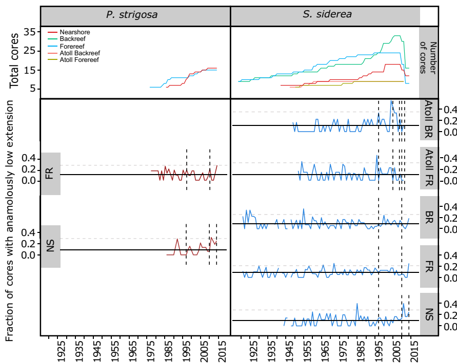
FIGURE 4 Total number of cores analyzed for each reef environment per species per year (top panel) and fraction of cores within each reef environment exhibiting anomalously low extension rates (i.e., annual extension rate in lowest 10% of cores) per year (bottom panel). Higher values in bottom panel indicate greater proportion of cores within a reef environment exhibiting anomalously low extension within a given year. Black horizontal lines indicate time-averaged ratios for each reef environment (separated by species). Horizontal dashed lines indicate the 95% confidence interval for the time-averaged ratios for each reef environment. Peaks that exceed this confidence interval represent significantly ( p < .05 ) higher percentages of corals exhibiting anomalously low extension rates in a given year. Vertical dashed lines indicate years in which Degree Heating Weeks \geq 4 for each reef environment (Table 2)
