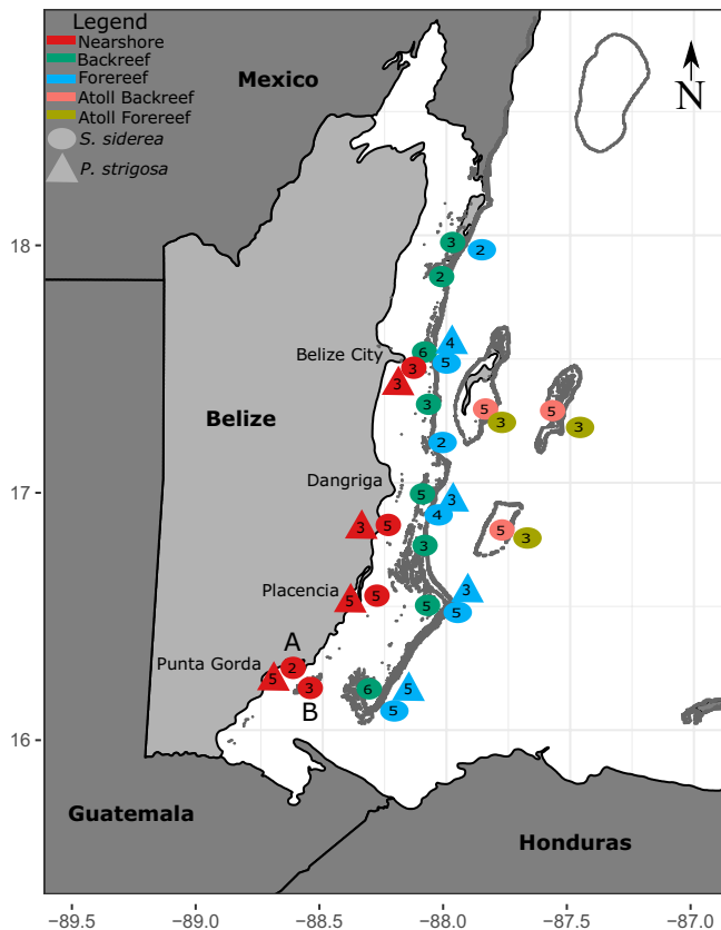
FIGURE 1 Map of reef sites on the Belize Mesoamerican Barrier Reef System where Siderastrea siderea and Pseudodiploria strigosa cores were extracted in 2009, 2012, and 2015. Circles and triangles represent core extraction sites for S. siderea and P. strigosa , respectively. Colors denote reef environment (nearshore = red, backreef = green, forereef = blue, atoll backreef = pink, and atoll forereef = yellow). Numbers denote total cores extracted for a particular species at a specific site
