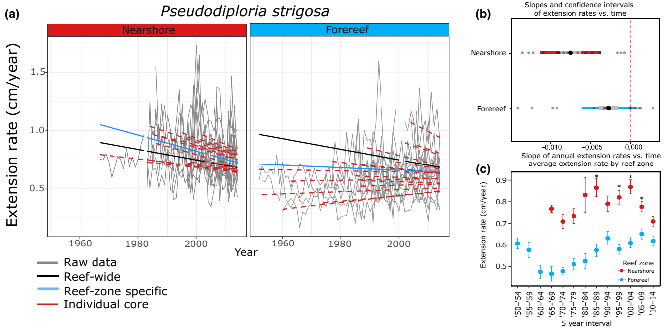
FIGURE 3 (a) Results of linear model of extension rate (cm/year) versus time for Pseudodiploria strigosa by reef environment for the 1950–present interval. Gray lines are raw extension data, black lines are average linear models of extension for all P. strigosa cores across all reef environments, blue lines are average linear models of extension for all P. strigosa cores within each reef environment, and red lines are linear models of extension for individual Siderastrea siderea cores within the reef environments. Raw (gray) and linearly modeled (red) extension chronologies highlight the variability in growth amongst colonies. (b) Slopes of linear models describe extension versus time for each reef environment, with small points representing individual cores and large points representing average slopes of all cores within a reef environment (gray bars and colored bars are 50% and 95% confidence intervals [CI], respectively, of average slope for each reef environment). Slopes are significantly different from each other if their 95% CI do not overlap. Likewise, slopes are significantly different from zero if their 95% CI do not overlap with the red dashed line centered on zero. (c) Five-year averages of skeletal extension rate by reef environment \pm 1 SE. Asterisks indicate statistically significant differences ( p < .05 ) between nearshore and forereef values
