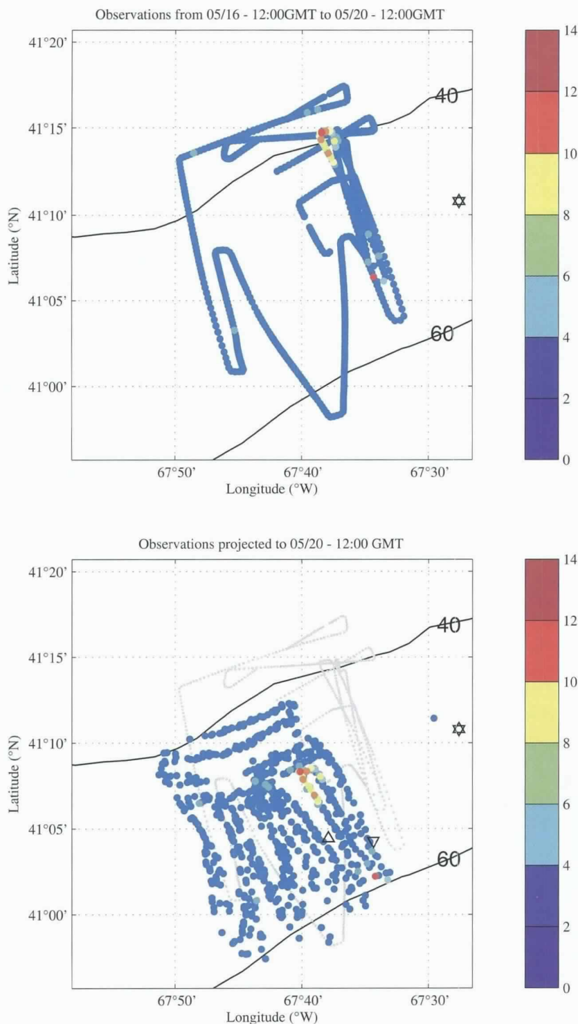
Figure 10. Model-based advective correction of dye observations. Top panel shows the location of the South Flank surface tracer release (star) and the track line of the first dye survey in geographic coordinates. The observed tracer concentration is indicated by dot color. Bottom panel shows the distribution of the same observations advected to the end of the survey (2.8 days after injection) by the modeled velocities. Also shown are the final positions of surface (upward-pointing triangle) and 15m (downward-pointing triangle) numerical drifters released in the solution at the site of injection. The grey dots indicate the original geographic locations of the observations.
