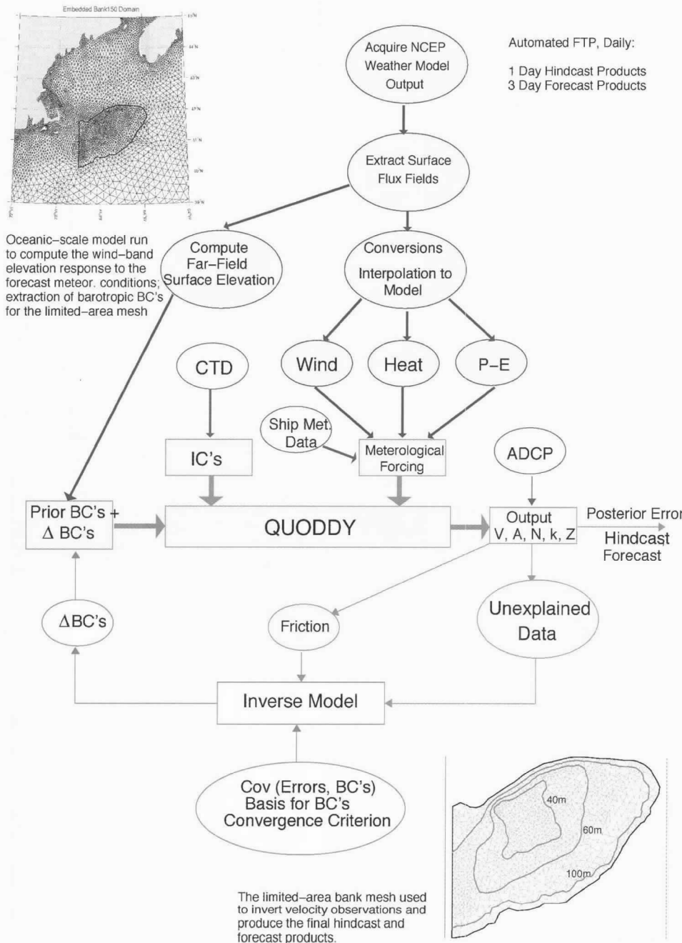
Figure 6. Iterative nonlinear inversion procedure. The oceanic forecast was computed on a wide-area domain (Westerink et al., 1992), forced by weather model forecasts and barotropic tides. Detided barotropic pressure was sampled on the bank-scale mesh boundary (outlined) and used to represent the far-field wind-band response as boundary conditions for the bank-scale calculation. The bank-scale forecast inverted local velocity data to improve boundary conditions. "QUODDY" (Lynch et al., 1996) is the basic simulation engine for the bank-scale. Iteration was used to accommodate its nonlinearities.
