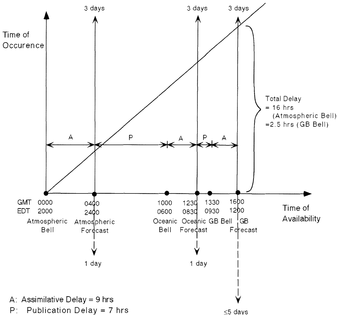
Figure 12. Timeline for cruise EN323, 324. The y-axis represents physical (natural) time; the x-axis represents the time of availability of information. A hindcast/forecast product is initiated at its bell time (closing time for relevant data) and published following an assimilation delay. A single daily cycle of three sequential forecasts is shown: the public weather model, operated by NCEP; the oceanic model, operated at the UNC shore station; and the Georges Bank model, operated at sea. Each calculation is represented by a vertical line (timeseries) at the point of its availability. The dotted line indicates the hindcast portion; the solid line, the forecast portion.
