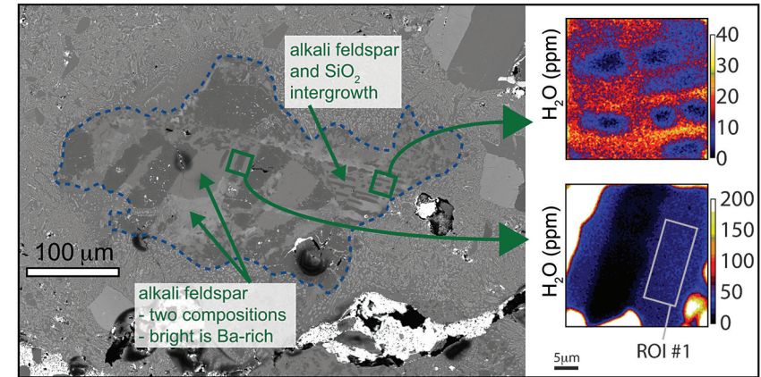
Figure 1 BSE image of granitoid clast (outlined in dashed line) from sample 15405,78, on the left. Clast consists of alkali feldspar and a silica phase. The variation in brightness of the feldspar relates to Ba ( i.e. bright has more Ba). On the right are chemical maps obtained by NanoSIMS at DTM. Water correlates with mineralogy. The alkali feldspar consistently has ~20 ppm H 2 O. The silica phase has similar water contents as the blank obtained on anhydrous glass (2–3 ppm).
