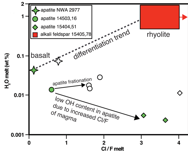
Figure 2 Plot of the estimated Cl/F ratio of magma versus estimated water content for lunar magmas (y-axis in log scale). Apatite data are from McCubbin et al. (2010). Water estimates from apatite assume 95 % crystallisation prior to apatite crystallisation. Cl/F melt estimates from apatite assume D_F/D_{Cl} is 10 (Webster et al. , 2009). Within individual samples, boundary layer crystallisation will create apatites with higher Cl and OH - contents than those initially growing from their host magma, thus the lowest water estimates from each sample (green fill) should be more representative of the initial magma composition (Boyce et al. , 2014). Schematic differentiation trend is shown between basalt and rhyolite. For reference, OH - data from apatites from lunar granite 14321,1047 (Robinson et al. , 2014) predict H 2 O melt compositions of 0.001 wt. %, and likely have Cl/F ratios higher than 3.
