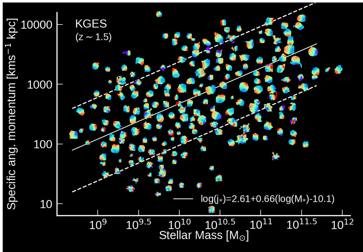
Figure 5. The H \alpha rotational velocity maps of the KGES galaxies with H \alpha signal to noise greater than 5, displayed in the specific stellar angular momentum stellar mass plane, offset to minimize overlap. The white solid line is a fit to the KGES data of the form \log_{10}(j_*) = \alpha + \beta(\log_{10}(M_*/M_\odot) - 10.10) , with the slope fixed to \beta = 0.66 and a derived intercept of \alpha = 2.61 . The white dashed lines are a factor of 10 above and below the fit. Low stellar mass, low angular momentum galaxies have smaller stellar continuum sizes and thus have a smaller extent of nebula emission compared to galaxies of higher stellar mass and higher angular momentum.
