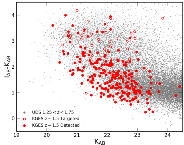
Figure 1. The observed ( I_{AB} - K_{AB} ) colour as a function of the observed K -band magnitude for the KGES sample. Galaxies detected in H\alpha are indicated by the red points (243 galaxies). The open symbols represent the 45 galaxies where the H\alpha signal to noise (S/N) is less than five. Star-forming galaxies in the UDS field in the redshift range 1.25 < z < 1.75 are shown for comparison (grey points).
