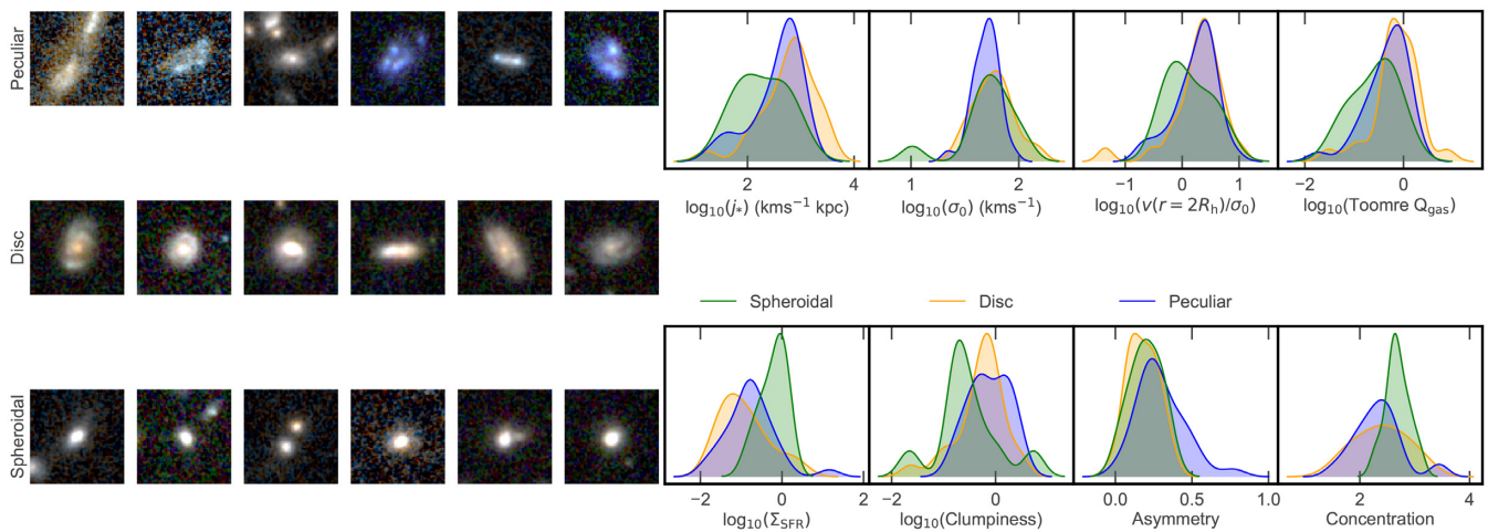
Figure 12. HST colour images of KGES galaxies. Spheroidal, disc, and peculiar morphological classes (left) with the kernel density distribution of specific angular momentum ( j_s ), velocity dispersion ( \sigma_0 ), ratio of rotation velocity to velocity dispersion ( V(2R_h)/\sigma_0 ), disc stability ( Q_{\text{gas}} ), H\alpha star formation rate surface density ( \Sigma_{\text{SFR}} ), clumpiness, asymmetry, and concentration (right). The velocity dispersion and concentration of spheroidal, disc, and peculiar galaxies are very similar. Spheroidal galaxies have lower specific stellar angular momentum, are more dispersion dominated, have lower Toomre Q_{\text{gas}} , are less clumpy, more asymmetrical but have higher \Sigma_{\text{SFR}} than disc-like galaxies. Peculiar galaxies on average have the same specific stellar angular momentum, are similarly rotation dominated, but have lower Toomre Q_{\text{gas}} and are more clumpy, more asymmetrical but with higher \Sigma_{\text{SFR}} than disc-like galaxies.
